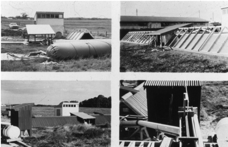
Figure 2 Pilot digester on research farm.
