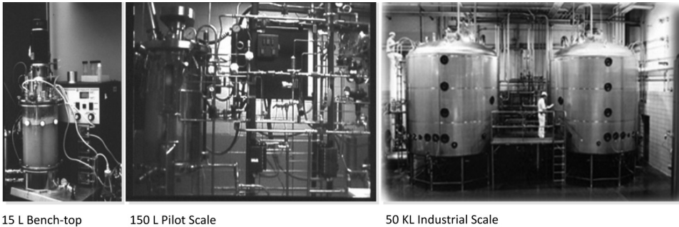
Figure 6 Production of keratinase by scaling up fermentation.
