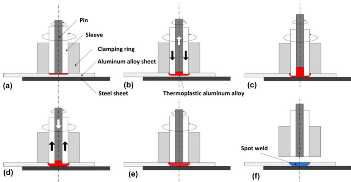
FIG. 7. Refill FSSW (a) before plunge, (b) plunge phase, (c) dwell phase, (d) refilling phase, (e) trim phase, and (f) retreating phase, with permission from Ref. 127.
