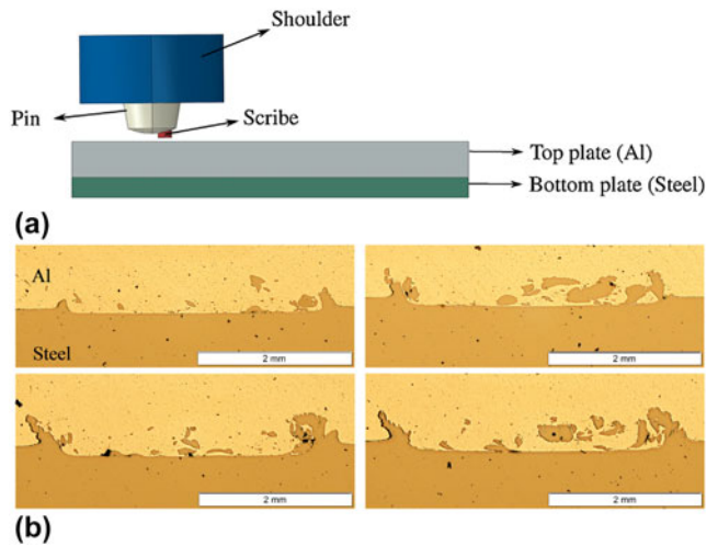
FIG. 8. (a) Friction stir scribe welding and (b) material mixing from friction stir scribe welding along the length, with permission from Ref. 144.
