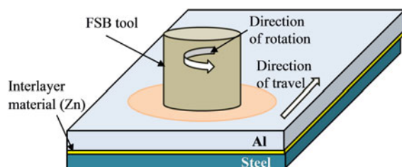
FIG. 9. Friction stir brazing of Al–steel.
