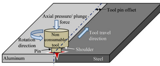
FIG. 4. Dissimilar FSW of steel to aluminum.
