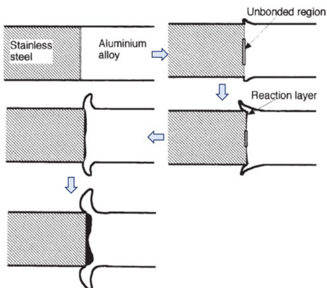
FIG. 2. Interlayer formation steps in dissimilar Al–steel friction welding, with permission from Ref. 42.
