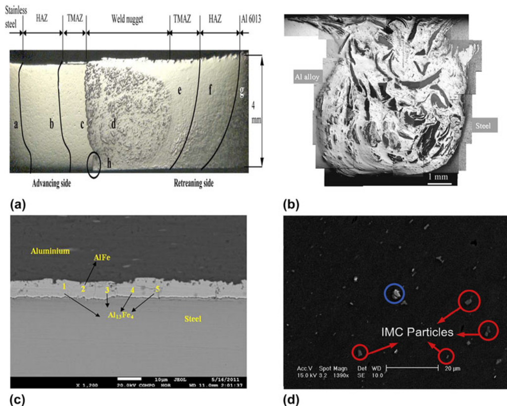
FIG. 5. Microstructural features of Al–steel FSW joints, (a) different zones indicated, with permission from Ref. 103, (b) complex stir zone, with permission from Ref. 102, (c) Al–steel interface with IMC layer, with permission from Ref. 107, and (d) presence of IMCs in the stir zone, with permission from Ref. 78.
