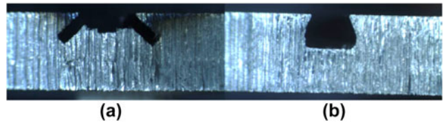
FIG. 11. Friction stir extrusion edge preparation (a) slit saw groove and (b) o ring dovetail groove, with permission from Ref. 150.
