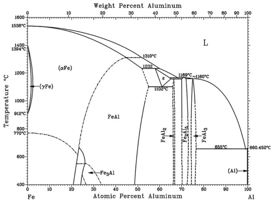
FIG. 1. Binary phase diagram of the Al–Fe system, with permission from Ref. 37.
