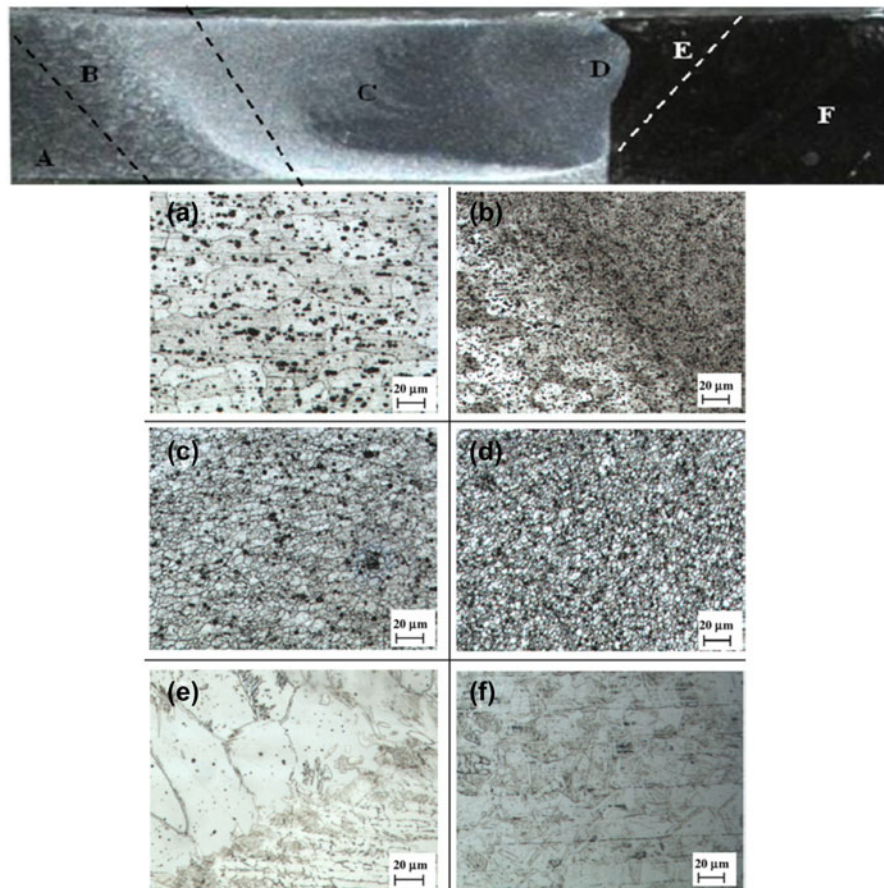
FIG. 6. Microstructural changes of dissimilar Al-steel GTAW assisted FSW joint: (a) Al base material, (b) TMAZ of Al side, (c) stir zone, (d, e) stir zone-steel interface-TMAZ of steel side, and (f) steel base material, with permission from Ref. 25.
