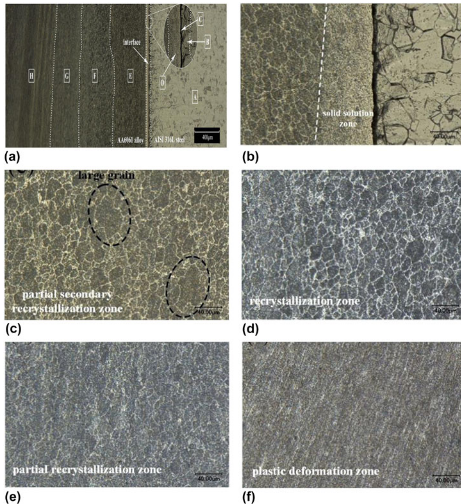
FIG. 3. Microstructural features of dissimilar Al–steel friction welds (a) Al–steel interface and different zones at Al sides, (b) solid solution zone at interface-region D of (a), (c) partial secondary recrystallized zone at Al-region E of (a), (d) recrystallized zone at Al-region F of (a), (e) partial recrystallized zone-region G of (a), (f) plastic deformation zone-region H of (a), with permission from Ref. 54.
