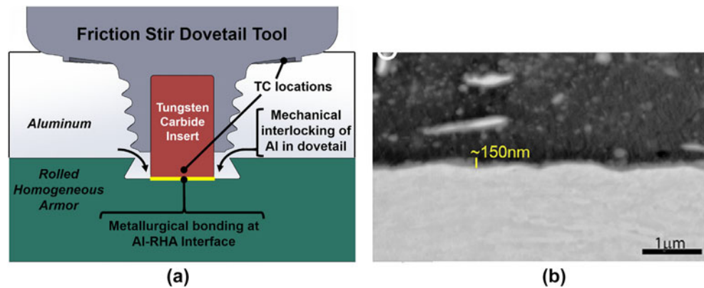
FIG. 12. Friction stir dovetailing (a) process description and (b) SEM image of joint interface, with permission from Ref. 152.
