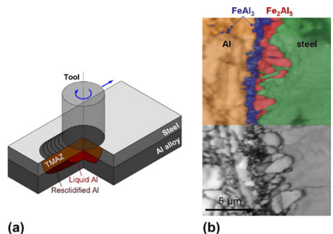
FIG. 10. Friction melt bonding (a) process principle and (b) formation of IMC-EBSD image, with permission from Ref. 147.
