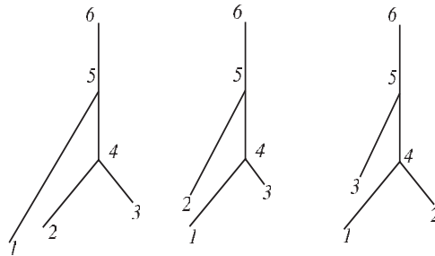
FIGURE 12. Morse trees with six vertices, three minima.
