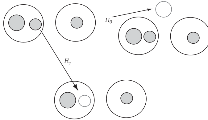
FIGURE 2. Attaching a 0-, 2-handle. The shaded areas indicate holes.
