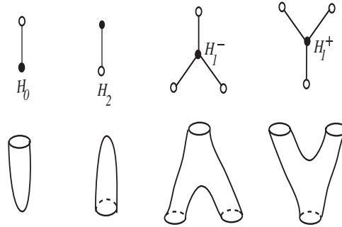
FIGURE 6. The elementary cobordism corresponding determined by the critical values.
