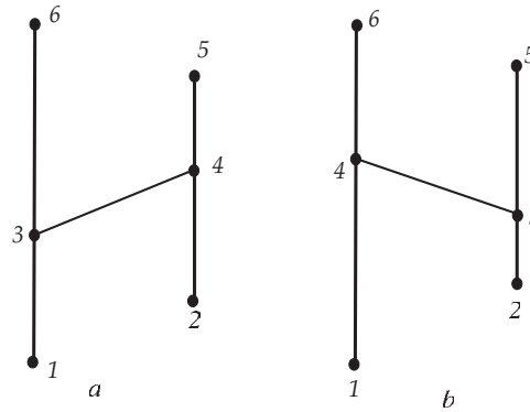
FIGURE 5. Morse trees of order two.
