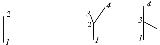
FIGURE 8. Cutting a Morse tree along the lowest H_1^- -handle.
