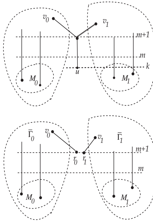
FIGURE 7. Cutting a Morse tree along the lowest H_1^+ -handle.
