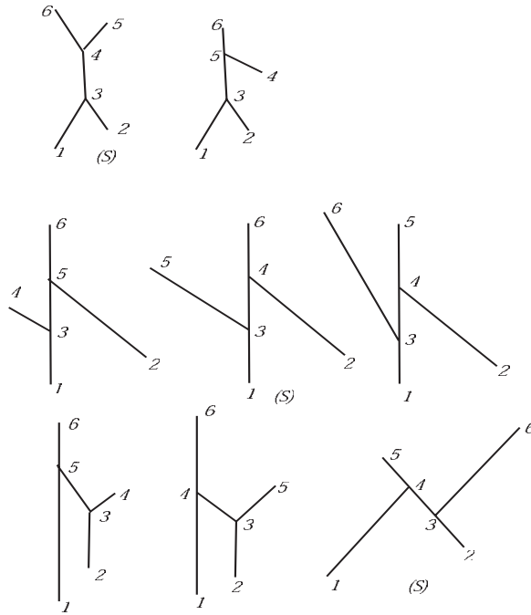
FIGURE 11. Morse trees with six vertices, and the first two are minima.
