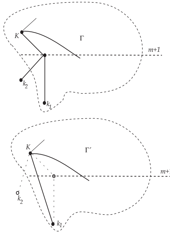
FIGURE 8. Cutting a Morse tree along the lowest H_1^- -handle.
