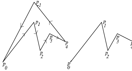
FIGURE 1. Cutting a Morse function down to a snake.
