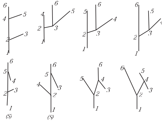
FIGURE 10. Morse trees with six critical points, and the second is a node.
