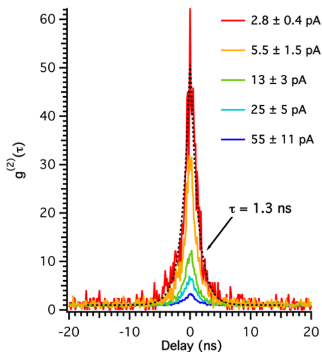
Figure 2. CL- g^{(2)} ( \tau ) of defects in h-BN for different excitation currents when there is more than one defect excited at the same time. A huge bunching effect ( g^{(2)}(0) \gg 1 ) is clearly visible.
