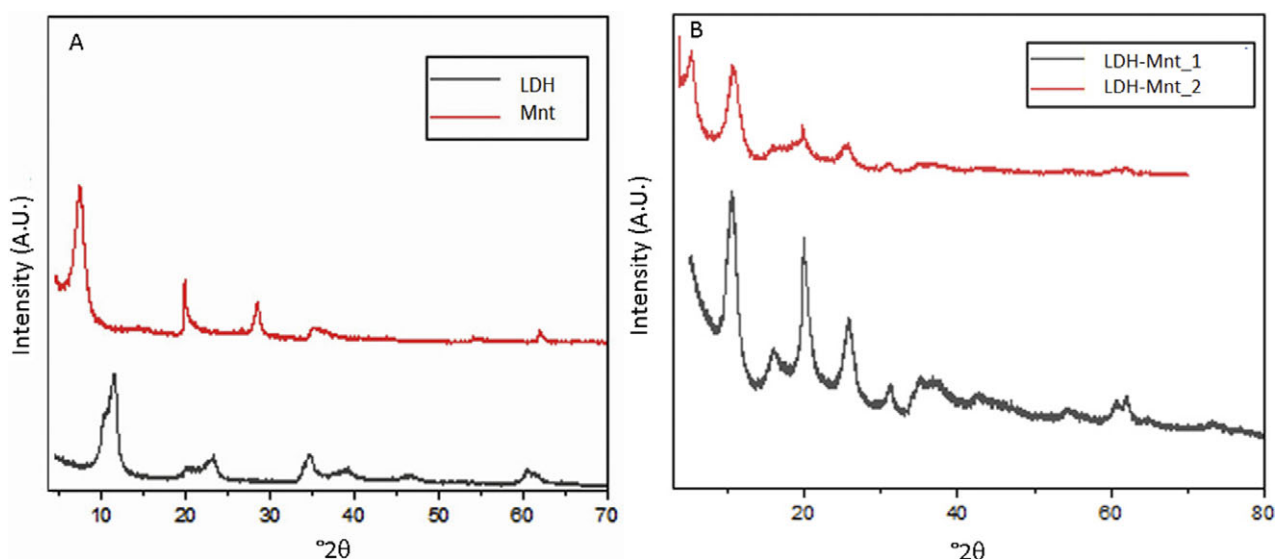
Figure 1. XRPD patterns of the samples: (A) LDH (black line) and Mnt (red line); (B) LDH-Mnt_1 (black line) and LDH-Mnt_2 (red line).
