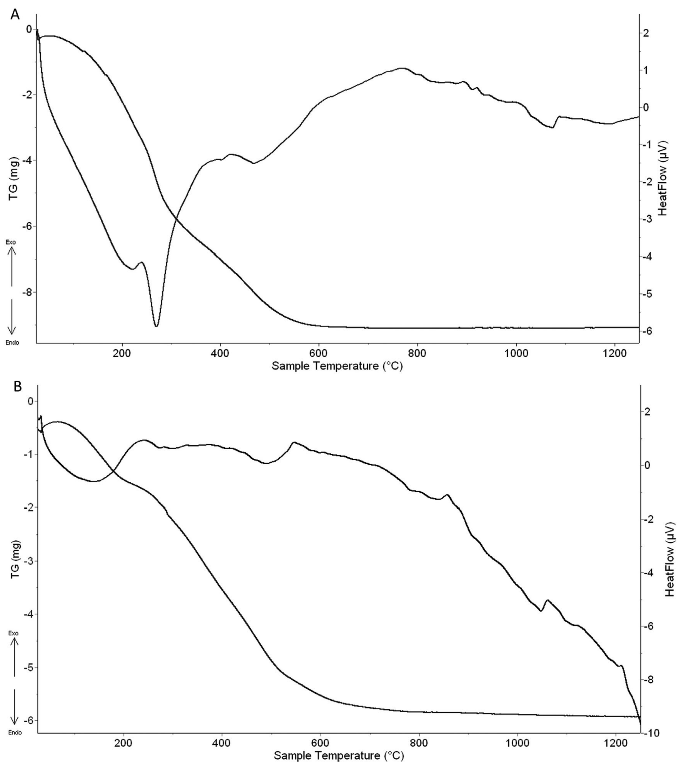
Figure 3. TG and heat-flow curves of: (A) LDH and (B) LDH-Mnt samples. Up and down arrows refer to exothermic and endothermic peaks, respectively.
