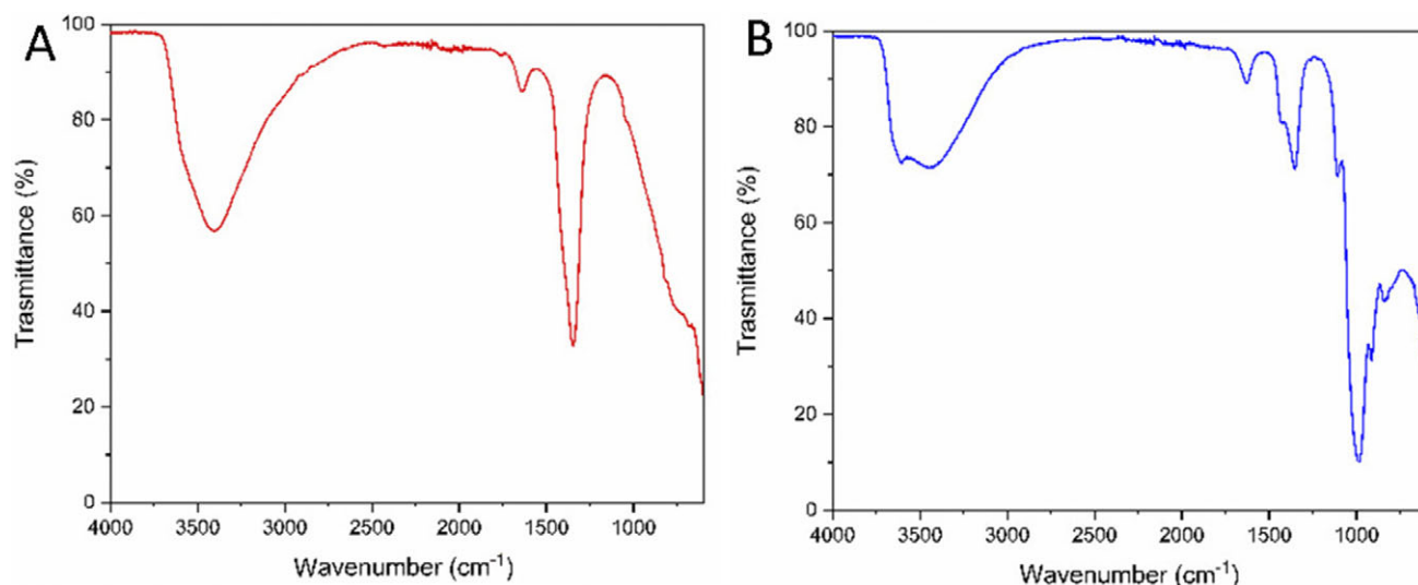
Figure 2. Infrared spectra of the samples: (A) LDH and (B) LDH-Mnt.
