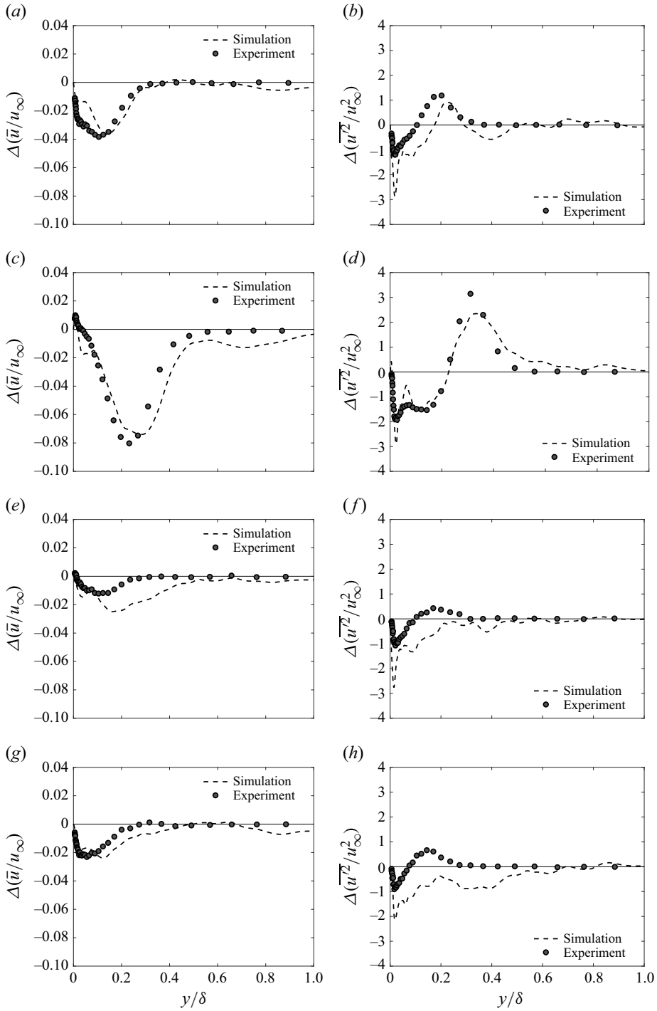
Figure 32. Comparison of \Delta \bar{u} and \Delta \bar{u}^2 between simulation and experiment at x/\delta = 2 downstream of the orifice centreline: (a) St_\delta = 2.3 , r = 0.45 , \Delta \bar{u} ; (b) St_\delta = 2.3 , r = 0.45 , \Delta \bar{u}^2 ; (c) St_\delta = 2.3 , r = 0.88 , \Delta \bar{u} ; (d) St_\delta = 2.3 , r = 0.88 , \Delta \bar{u}^2 ; (e) St_\delta = 0.5 , r = 0.3 , \Delta \bar{u} ; (f) St_\delta = 0.5 , r = 0.3 , \Delta \bar{u}^2 ; (g) St_\delta = 1.5 , r = 0.3 , \Delta \bar{u} ; (h) St_\delta = 1.5 , r = 0.3 , \Delta \bar{u}^2 .
