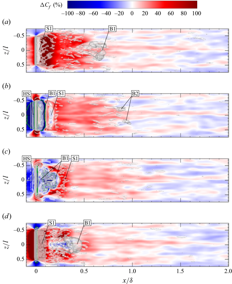
Figure 27. \Delta C_f spatial map overlaid with isocontours of Q = 2 \times 10^{-3} U_\infty^2/\delta^2 for four phases for the St_\delta = 0.5, r = 0.3 case: (a) \phi = 0 ; (b) \phi = \pi/2 ; (c) \phi = \pi ; (d) \phi = 3\pi/2 .
