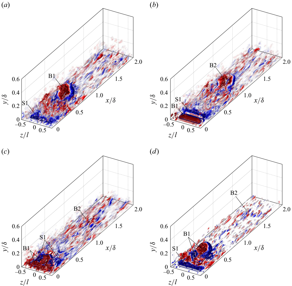
Figure 23. Isometric views of isocontours of Q = 6 \times 10^{-4} U_\infty^2 / \delta^2 and Q = 2 \times 10^{-4} U_\infty^2 / \delta^2 (translucent) for four phases for the St_\delta = 0.5 , r = 0.3 case: (a) \phi = 0 ; (b) \phi = \pi/2 ; (c) \phi = \pi ; (d) \phi = 3\pi/2 .
