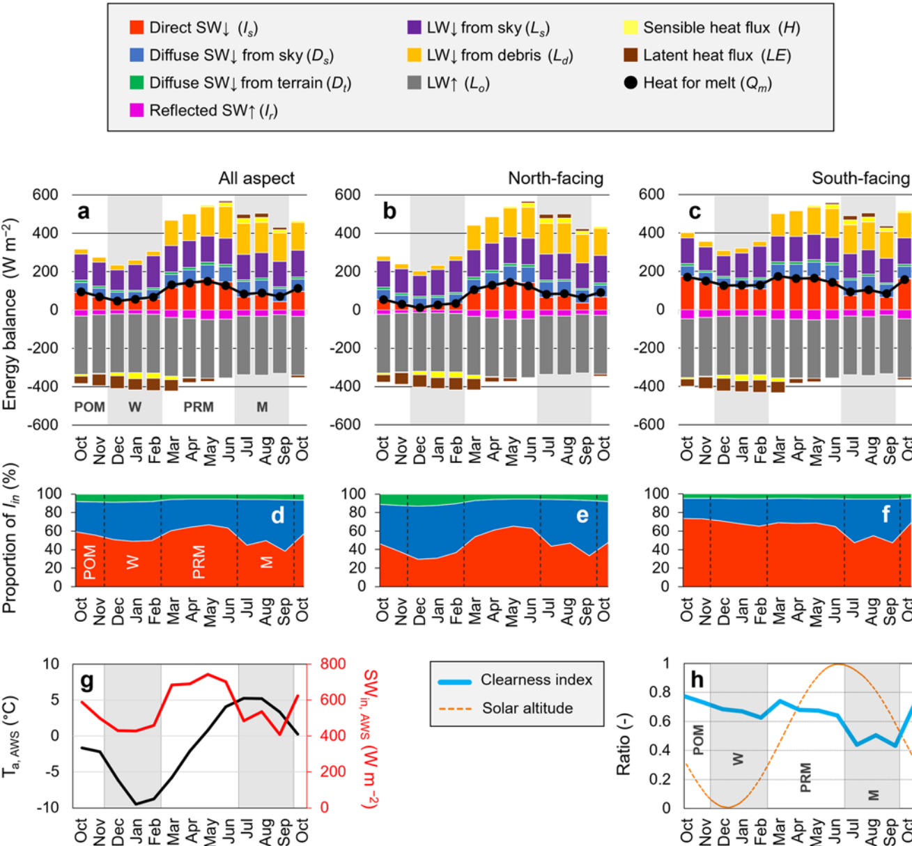
Figure 10. Mean energy balance of all (a), north-facing (b), and south-facing (c) ice cliffs. Components of incoming shortwave radiation ( i_s , d_s , and d_t ) of all (d), north-facing (e), and south-facing (f) ice cliffs. (g) Observed air temperature ( t_{a, AWS} ) and incoming shortwave radiation ( sw_{in, AWS} ) at the AWS. (h) Clearness index at the AWS (section 2.4) and normalised solar altitude for Trakarding Glacier. Note that almost of the melt of ice cliffs were occurred in daytime. During the time steps when the energy balance became negative, the heat for ice cliff melt ( q_m ) was treated as zero.
