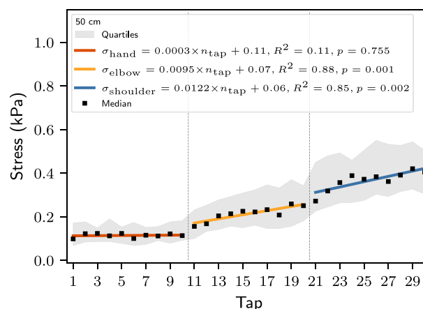
Figure 7. Median stress levels and their interquartile ranges for the measurements at 50 cm depth.
