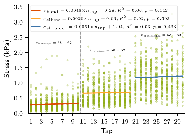
Figure 10. Stress levels for the different taps by different people under no-snow conditions.
