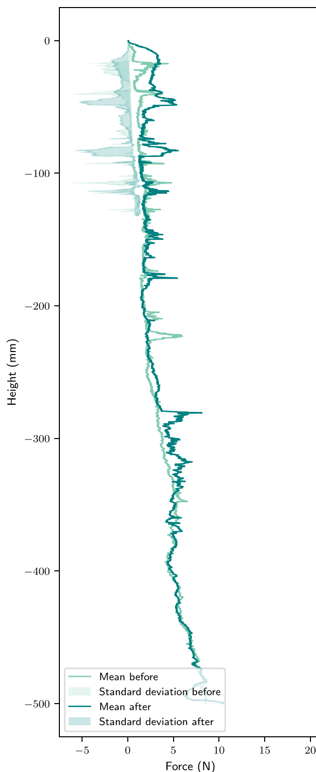
Figure 9. Average SMP resistance and standard deviation of all CTs at Weissfluhjoch before (11 profiles) and after (ten profiles) the CT as a function of snow depth.
