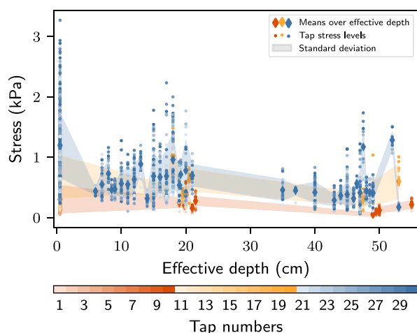
Figure 8. Average stress levels and their standard deviation as a function of effective depth.
