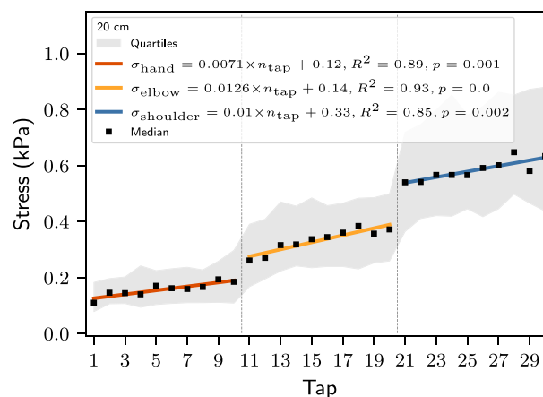
Figure 6. Median stress levels and their interquartile ranges for the measurements at 20 cm depth.
