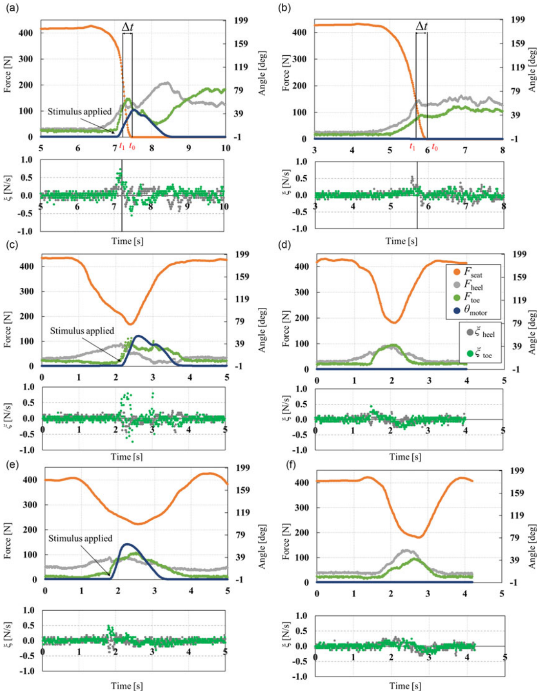
Figure 15. Example figure comparing the online test results for the three types of motions performed by Subject #1. The figure shows the time-based changes in F_{heel} , F_{toe} , \xi_{heel} , \xi_{toe} , \theta_{motor} (with the initial rotation indicating when the toe pedal began to rotate), and F_{seat} . (a) (b) Normal STS motion with and without a stimulus. (c) (d) Grabbing items in front with and without a stimulus. (e) (f) Picking up an item from the ground with and without a stimulus.
