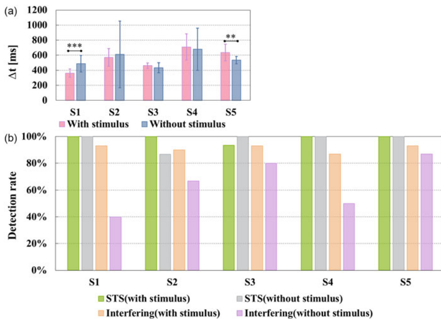
Figure 19. Online test results under conditions with and without stimulus for five subjects (S1–S5 denote Subject #1 through to Subject #5), using thresholds from points on the Pareto front where the detection rate of interfering motions is equal to 1. (a). Advance detection time \Delta t (b). Detection rates of STS motion and interfering motions under both conditions. Statistical significance is indicated as follows: ** p < 0.01 , *** p < 0.001 .
