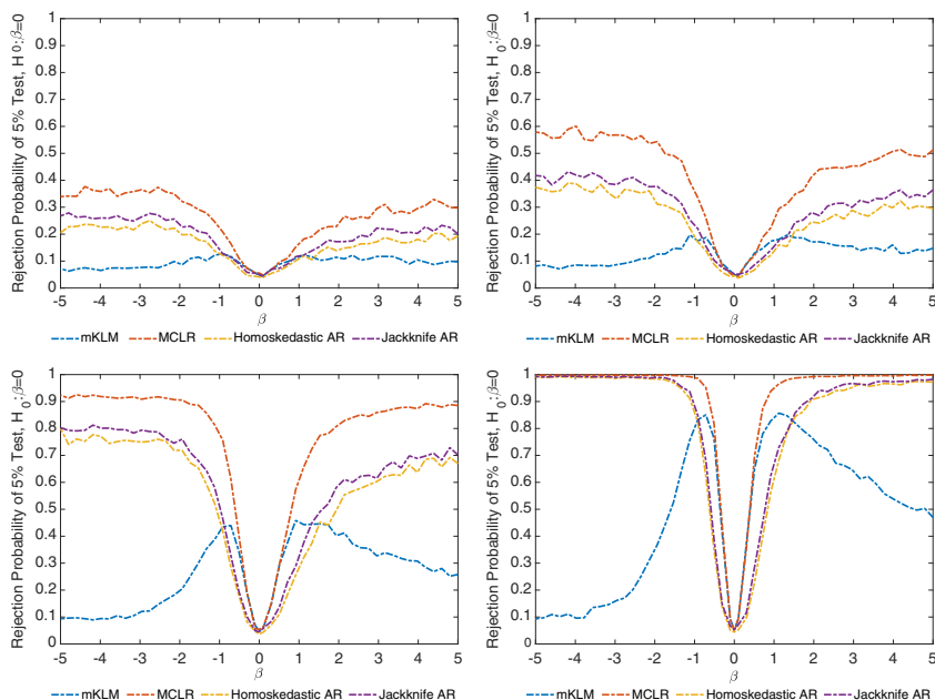
FIGURE 2. Calibrated power curves.
