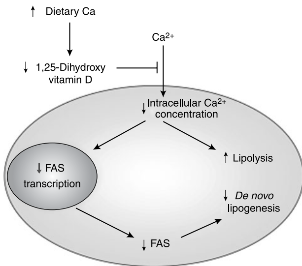
Fig. 2. Hypothesised mechanism of stimulation of lipolysis and inhibition of lipogenesis by dietary Ca. Increased dietary Ca intake lowers the level of the hormone 1,25-dihydroxy vitamin D, thereby lowering the uptake of \text{Ca}^{2+} into the cell. Decreased levels of intracellular Ca stimulate lipolysis and decrease the transcription of fatty acid synthase (FAS), resulting in the inhibition of lipogenesis.
