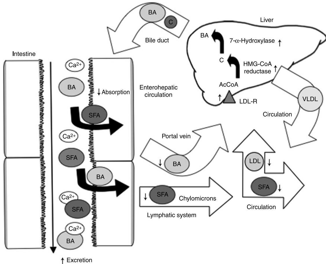
Fig. 1. One of the proposed mechanisms of action of dietary Ca. Ca binds to SFA or bile acids (BA) in the intestine, inhibiting their absorption. SFA raise LDL-cholesterol, probably by decreasing LDL-receptor (LDL-R) activity. Reduced absorption of SFA can therefore lower serum LDL-cholesterol. In the liver, cholesterol is converted into BA. Lowering the absorption of BA in the intestine will therefore lead to an increased conversion of cholesterol and reduced serum LDL-cholesterol levels. C, cholesterol; ↑, increased; HMG, 3-hydroxy-3-methyl-glutaryl; ↓, reduced; AcCoA, acetyl-CoA.
