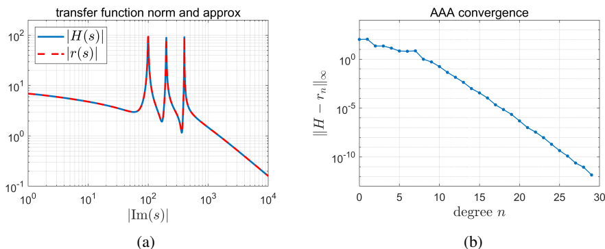
Figure 19.1. (a) Absolute values of the degree 1006 transfer function H(s) and its degree 29 AAA approximant r(s) for the FOM example from SLICOT (Chahlaoui and Van Dooren 2002). (b) AAA convergence for this example. Rapid convergence begins at degree n = 6 , after the six poles at -1 \pm 100i , -1 \pm 200i and -1 \pm 400i are captured.
