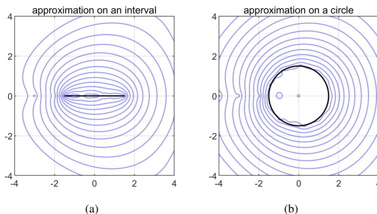
Figure 3.2. AAA approximation of \Gamma(z) based on samples at (a) 50 Chebyshev points in [-1.5, 1.5] and (b) 50 equispaced points on |z| = 1.5 . From inside out, the contours represent relative errors |r(z) - \Gamma(z)|/|\Gamma(z)| = 10^{-13}, 10^{-12}, \dots, 10^{-1} .
