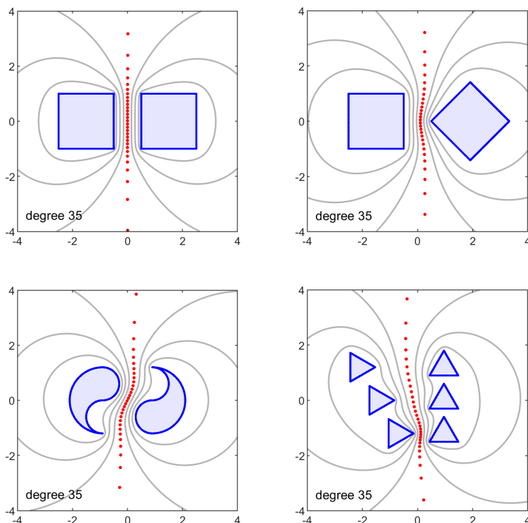
Figure 20.3. Four more examples of AAA-Lawson minimax solutions of the Zolotarev sign problem, all for fixed degree 35. The 'sign' and 'damping' options have been used with a damping factor \delta = 0.95 . The contours mark accuracies 10^{-9} , 10^{-6} and 10^{-3} .
