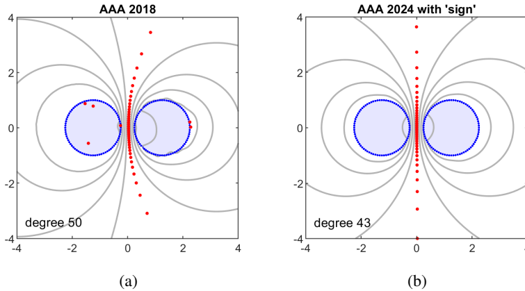
Figure 20.1. Approximation of \text{sign}_{E/F}(z) for a pair of disks discretized by 80 equispaced points on each boundary. Standard AAA does poorly on such problems (a), whereas AAA with the 'sign' modification introduced in 2024 and described in Trefethen and Wilber (2025) does much better (b). The grey contours mark deviations 10^{-12} , 10^{-9} , 10^{-6} and 10^{-3} of r(z) at each point z from +1 or -1 , whichever is closer.
