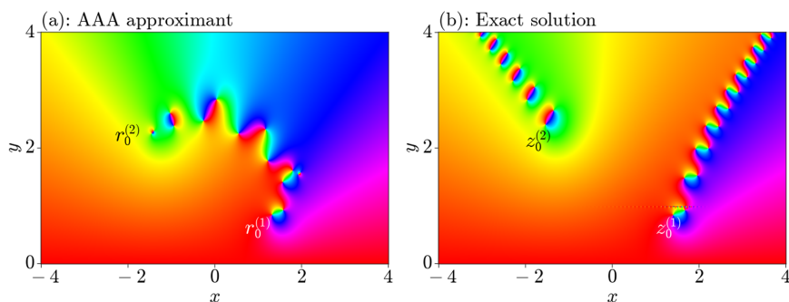
Figure 14.3. A figure comparing the exact pole structure of a Burgers solution with its AAA approximation from data on the real axis. The poles closest to the axis are accurately captured, but not the poles further out. (Note that the real and imaginary axes in these images are not equally scaled.) This figure is not part of the governing Open Access licence for the article but has been reproduced from VandenHeuvel et al. (2023) © (2023), with permission from Elsevier, www.elsevier.com .
