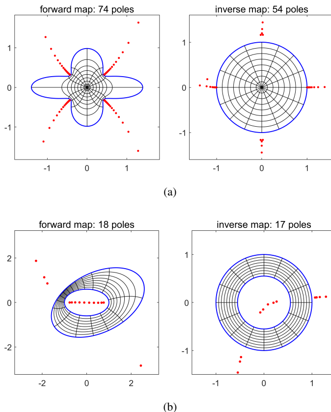
Figure 25.1. (a) Conformal map computed by Chebfun conformal from a smooth cross-shaped domain to a disk, and its inverse. Each map is represented to 9-digit accuracy by a rational function obtained by AAA, and can be evaluated in about 0.5 \mu\text{s} per point. (b) Doubly connected conformal map computed by Chebfun conformal2 and its inverse. Each map is represented to 7-digit accuracy by a rational function obtained by AAA, and can be evaluated in about 0.1 \mu\text{s} per point.
