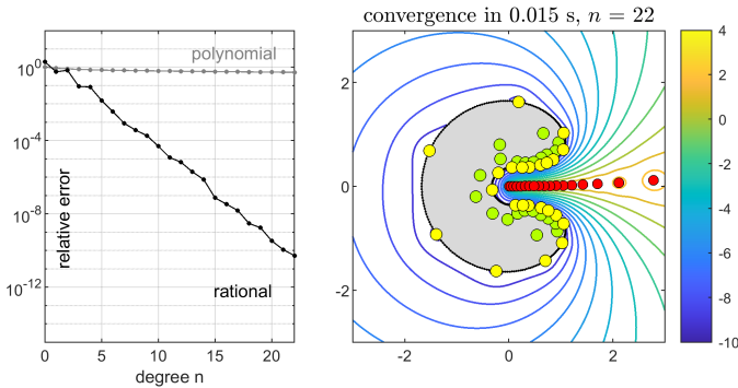
Figure 12.5. Approximation of f(z) = \log(-z) on a non-convex region. Both polynomials and rational functions converge exponentially, but at vastly different rates (Trefethen 2024).
