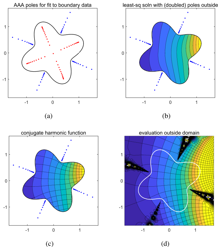
Figure 24.1. Illustration of AAA-least squares (AAALS) for a Laplace Dirichlet problem on a smooth non-convex domain \Omega with boundary data h(z) = \exp(\operatorname{Re}(z)) . First h is approximated by a complex rational function r with poles inside and outside \Omega . The poles inside are discarded, and the poles outside are taken as the locations of second-order poles for a least-squares fit to h by the real part of a rational function of degree 114. In this example 12-digit global accuracy is achieved in about 1/4 s on a laptop; we estimate the value at the centre as u(0) \approx 1.2157681370405 . The same accuracy with a polynomial fit would require a degree in the thousands, which would increase to millions for slightly deeper indentations.
