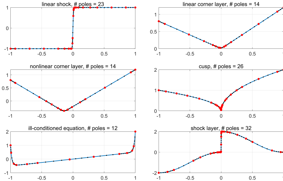
Figure 13.1. Solutions to the six singularly perturbed ODE boundary-value problems from Examples 91–96 of Appendix B of Trefethen et al. (2018) approximated to 6-digit accuracy by AAA rational approximations computed by the continuum AAA algorithm of Section 30. Red dots mark adaptively determined support points, and black dots mark additional sample points. Despite the narrow layers, the fits are of low degrees, suggesting a strong potential for efficient rational function solution of difficult ODEs if a suitable algorithm can be developed.
