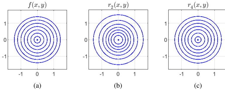
Figure 15.1. (a) Contours |f(x, y)| = 0, 0.2, 0.4, \dots, 1.4 of the bivariate function (15.1). (b,c) The same contours for the degree 2 and 4 rational approximations (15.2) and (15.3). No numerical approximation algorithm is known for finding near-best multivariate rational approximations like these.
