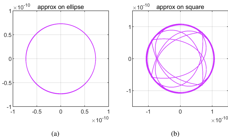
Figure 29.2. Error curves for two more degree 11 AAA-Lawson approximations of \Gamma(z) . (a) The domain is the ellipse with extreme points \operatorname{Re} z = \pm 1.5 and \operatorname{Im} z = \pm 2 and the error curve is very nearly circular. (b) The domain is the square -1.5 \leq \operatorname{Re} z, \operatorname{Im} z \leq 1.5 , and the four corners are visible in the error curve. The winding numbers are 18 (a) and 19 (b).
