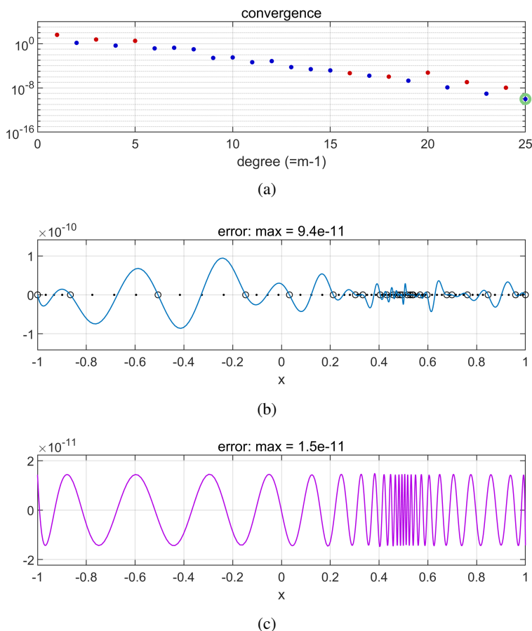
Figure 30.1. Continuum AAA near-best rational approximation of f(x) = \log(1 + 1000(x - \frac{1}{2})^2) on [-1, 1] . The convergence curve in plot (a) shows red dots at degrees with ‘bad poles’ in [-1, 1] and blue dots at degrees without such poles. Plot (b) shows the final degree 25 AAA error curve, with adaptively determined support points marked by circles and other sample points by dots. Plot (c) shows the error curve for a best approximation of the same degree computed by continuum AAA-Lawson.
