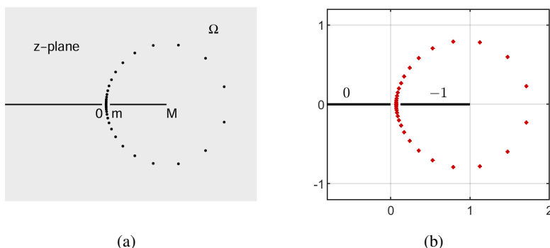
Figure 22.3. (a) A figure showing quadrature nodes derived by conformal mapping for a problem of computing functions of matrices with eigenvalues in [m, M] . © SIAM, reproduced with permission from Hale et al. (2008) . (b) A figure adapted from Horning and Trefethen (2025) showing nodes derived by a rational approximation of the Zolotarev sign type. The accuracy of the two formulas is comparable.
