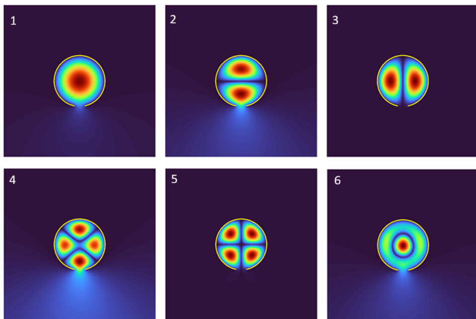
Figure 16.1. Images of the first six complex resonances in the unit disk with a gap in the boundary of angle \pi/8 . Images 2–3 and 4–5 are near-degenerate pairs that become exactly degenerate in the limit of zero gap size. © SIAM, reproduced with permission from Bruno et al. (2024).
