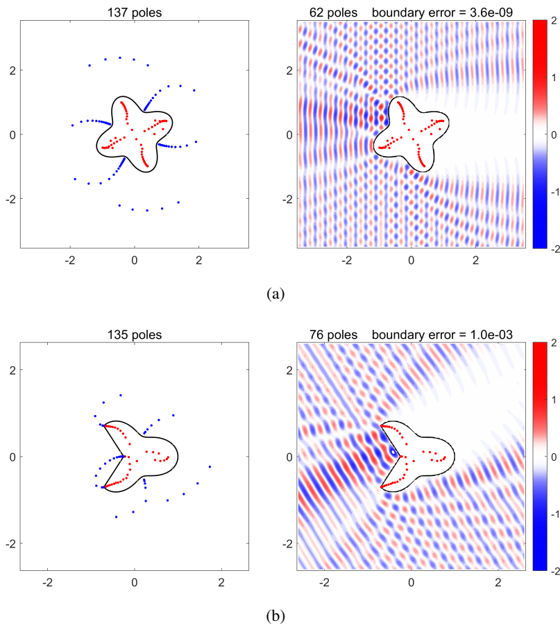
Figure 26.1. (a) A AAA-Helmholtz scattering computation with k = 20 for the domain of Figure 24.1; the real part of the complex solution u(z) is plotted. (b) A similar calculation for the domain of Figure 24.2. Here the incident wave has been rotated to an angle aligned with one of the straight boundary segments, causing strong reflection in that direction – amplitudes \approx \pm 2 associated with constructive interference.
