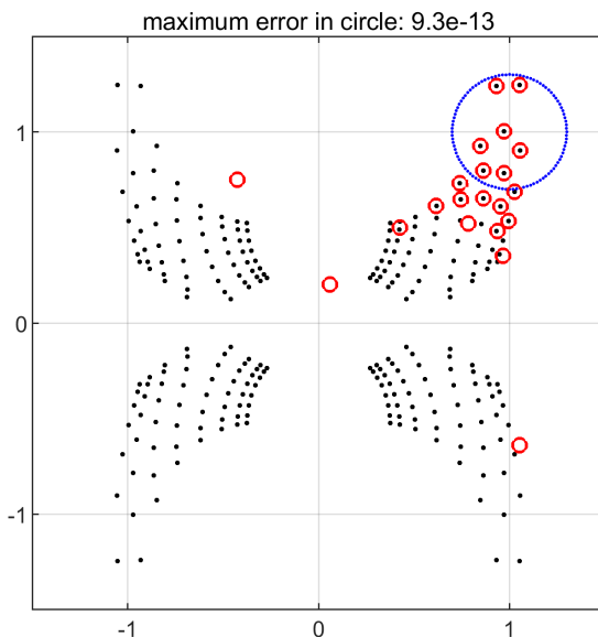
Figure 18.1. Calculation of 7 nonlinear eigenvalues of the ‘butterfly’ problem from the NLEVP collection (Betcke et al. 2013). AAA approximation is based on 100 samples on the circle |z - (1 + i)| = 0.3 , shown in blue. Black dots mark all the eigenvalues for this problem, and red circles show the AAA poles.
