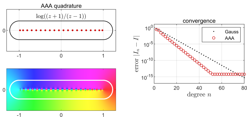
Figure 22.2. Like Figure 22.1, but now the quadrature formulas are based on approximation of \log((z+1)/(z-1)) over the boundary of an \varepsilon -neighbourhood of [-1, 1] . For the same test integrand f(z) = 1/(1+20z^2) as before, the convergence is about \pi/2 times faster than with Gauss quadrature, and the quadrature nodes are much more evenly spaced.
