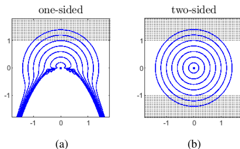
Figure 15.2. Bivariate approximation of (15.1) by AAA approximation along vertical lines. (a) Approximation along vertical lines with data samples just above the singularity, marked by black dots. (b) Approximation along vertical lines with samples on both sides of the singularity.
