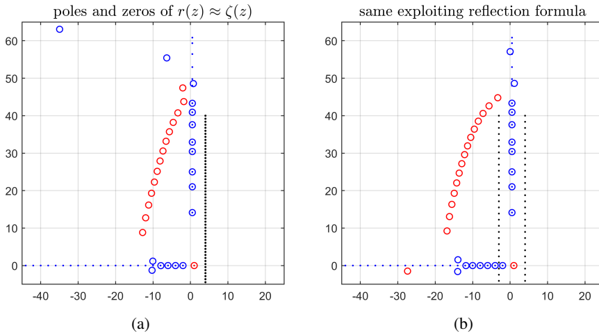
Figure 4.2. (a) Poles (red circles) and zeros (blue circles) of the degree 29 AAA approximation of the Riemann zeta function \zeta(z) based on sample values at 100 points with \text{Re } z = 4 (black dots). The pole and the zeros of \zeta(z) are marked by red and blue dots, respectively. The pole of \zeta(z) is captured to 11 digits of accuracy, whereas the other poles of r(z) are artifacts of the approximation (red circles). The first few zeros of \zeta(z) on the critical line \text{Re } z = 1/2 are also highly accurate. This figure shows the upper half of a symmetric configuration in the complex plane. (b) The same except with 50 sample points in the right half-plane and also their reflections by (4.4) in the left half-plane. The rational approximation is now of degree 32; the accuracy is similar.
