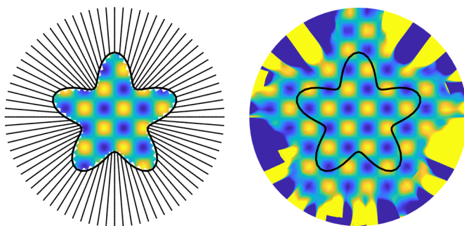
Figure 15.3. Continuation of a smooth function across a boundary by univariate AAA approximation on 60 radial lines. As in Section 10, about one wavelength of accurate extension is achieved. Figure reproduced from Trefethen (2023), licensed under CC BY-4.0.
