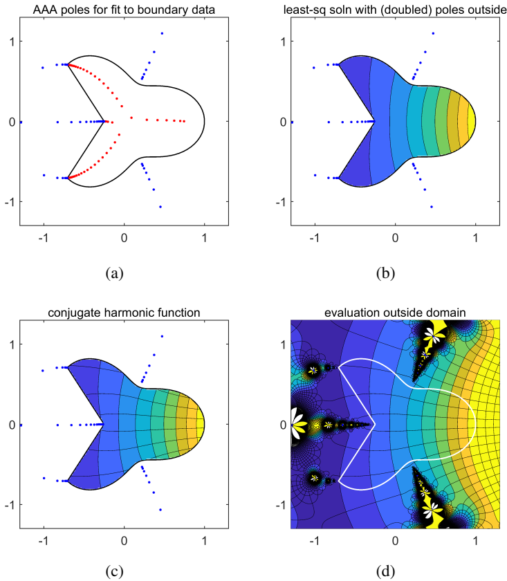
Figure 24.2. Repetition of Figure 24.1 for a harder problem with both corner singularities and non-convexity. The global accuracy is about 7 digits, and the value at the centre is u(0) \approx 1.081415507437 .
