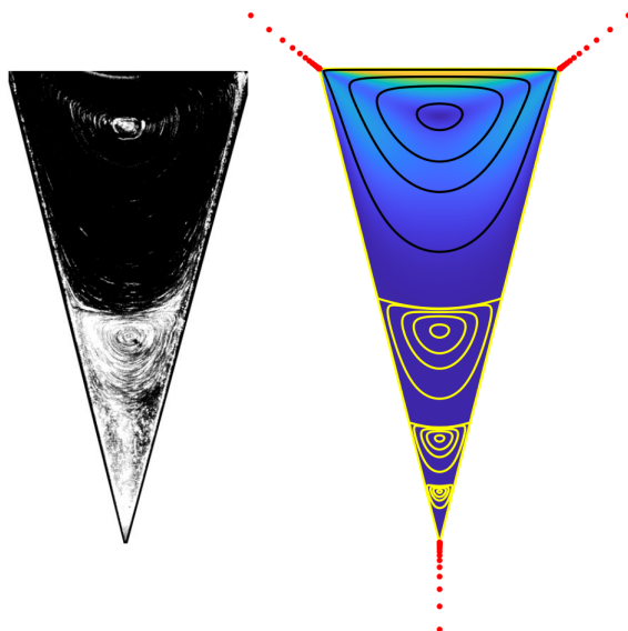
Figure 27.1. Figure showing Stokes flow in a triangular driven cavity computed by the lightning Stokes method. No-slip boundary conditions are applied everywhere, with the top boundary moving at constant speed and the remainder of the boundary stationary. The red dots are poles placed near each corner according to the lightning a priori clustering formula. The yellow contours mark the first three of an infinite series of counter-rotating Moffatt eddies, each with amplitude about 830 times less than the one above. © SIAM, reproduced with permission from Brubeck and Trefethen (2022). On the left, a laboratory experiment in the same configuration from Taneda in 1979 reproduced in An Album of Fluid Motion (Van Dyke 1982).
