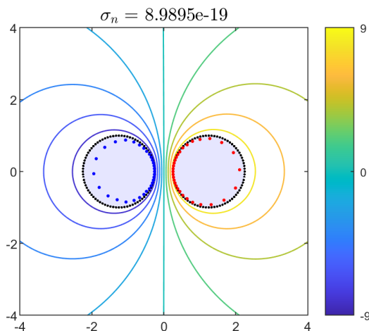
Figure 21.1. Approximation to the degree n = 30 solution r_n^* of the Zolotarev ratio problem for the two-disk configuration of Figures 20.1 and 20.2. This is a transformation of the function \hat{r}_n of Figure 20.2(b) by the formula (21.4). Blue and red dots mark zeros and poles of the computed r_n^* (the exact results would coalesce at two points), and the contours mark level curves of \log_{10} |r_n^*(z)| .
