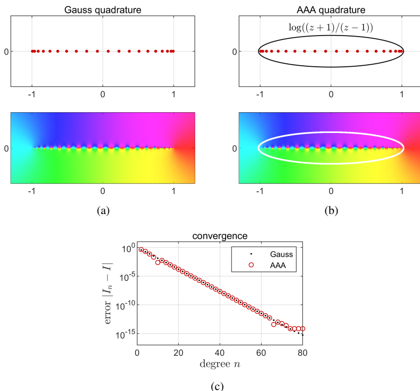
Figure 22.1. (a) Nodes for the 20-point Gauss quadrature formula and a phase portrait of the associated rational function (22.3). (b) Looking virtually identical, the same plots for a degree 20 AAA rational approximation of \log((z+1)/(z-1)) on a Bernstein ellipse. (c) Convergence of the two quadrature formulas for the test integrand f(x) = 1/(1+20x^2) .
