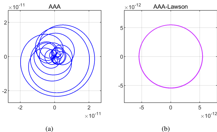
Figure 29.1. Repetition of Figure 3.3, but with the degree n of the AAA approximation of \Gamma(z) on the circle |z| = 1.5 reduced from 12 to 11 to stay well above the level of rounding errors. (a) The error curve for AAA near-best approximation passes through the origin n + 1 = 12 times, at each of the support points. (b) The error curve for AAA-Lawson best approximation is a near-circle of winding number 2n - 3 = 19 . Note the different scales on the two sides, reflecting the pattern that best approximations typically have errors smaller than those of AAA approximations by a factor less than 10.
