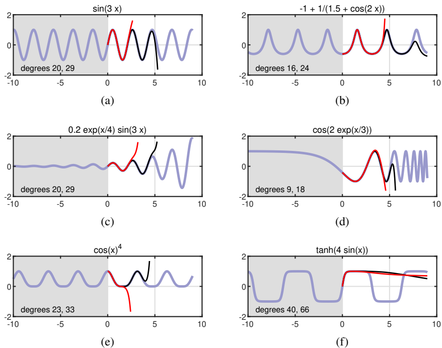
Figure 10.2. Illustration of the ‘one-wavelength principle’ by six examples in which an analytic function f(x) is analytically continued by AAA approximation from data for x \in [-10, 0] to x > 0 . The thick blue-grey curves show f(x) , the red curves show approximations r(x) with 13-digit accuracy, and the black curves show approximations r(x) with 29-digit accuracy. Approximately one and two wavelengths of successful continuation, respectively, appear to be achieved at least in the first four cases.
