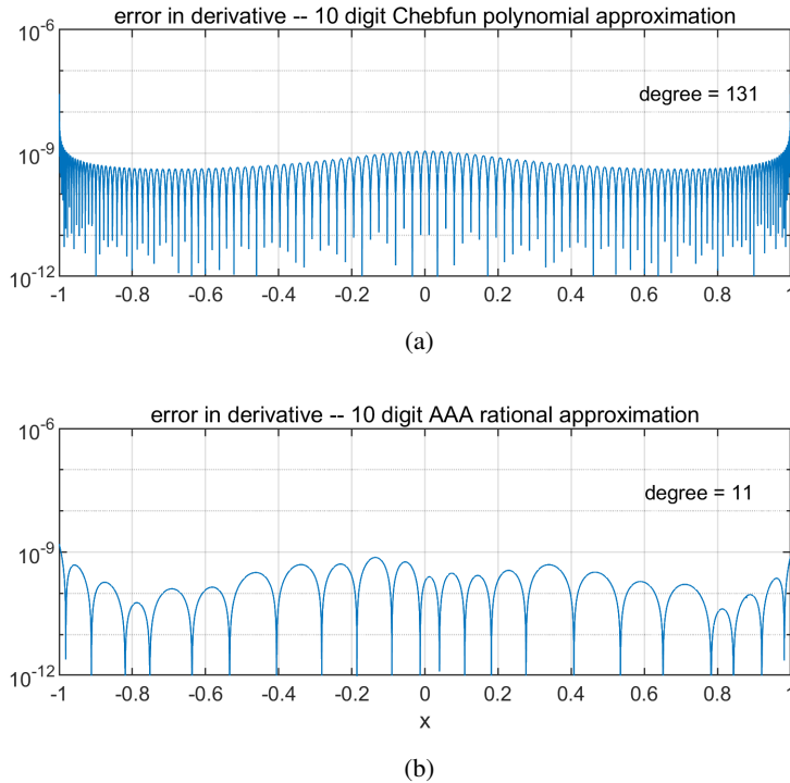
Figure 5.1. Numerical computation of the derivative of f(x) = \tanh(8x) for x \in [-1, 1] based on polynomial and rational approximations of f accurate to 10 digits. For f(x) = \tanh(80x) , the degrees increase to 1201 and 22.
