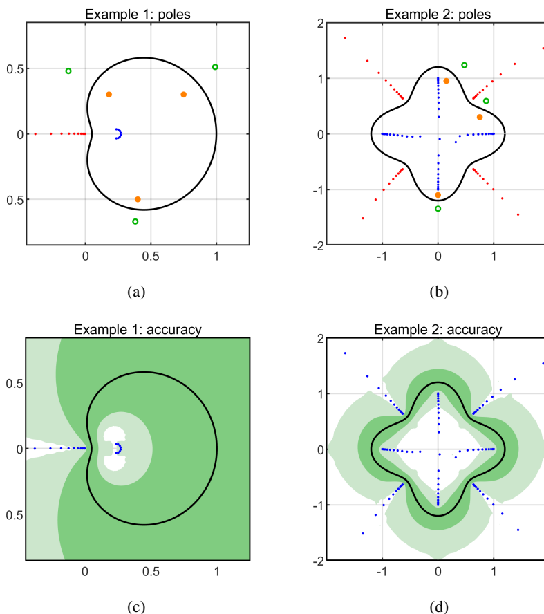
Figure 11.2. Numerically computed Schwarz functions for closed curves \Gamma obtained as images of the unit circle under maps f : (a,c) f(z) = \exp(1.5(z - 1)) , and (b,d) f(z) = z(1 + 0.2 \cos(4 \arg(z))) . (a,b) The dots show poles of the AAA approximants, blue for poles inside \Gamma and red for poles outside. The orange/green dots illustrate three arbitrary pairs of points mapped to each other by \overline{S(z)} . (c,d) As a test of (11.3), dark and light green shading indicates regions where |\overline{S(\overline{S(z)})} - z| is less than 10^{-8} and 10^{-1} , respectively.
