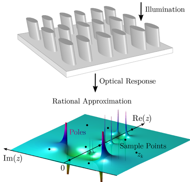
Figure 18.2. Image suggesting the use of AAA approximation to calculate nonlinear eigenvalues in photonics applications. Figure reproduced from Betz et al. (2024) , licensed under CC BY-NC-ND 4.0.
