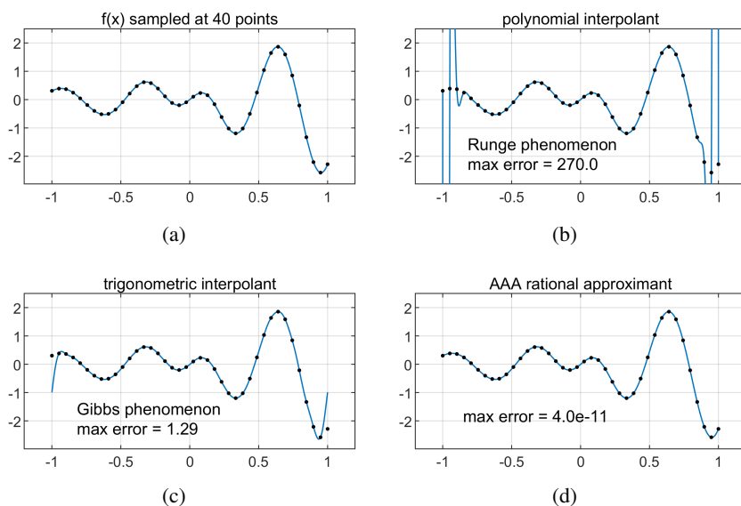
Figure 8.1. For interpolation of non-periodic equispaced data, polynomials suffer from the Runge phenomenon and trigonometric polynomials from the Gibbs phenomenon. The best general-purpose method appears to be AAA approximation.
