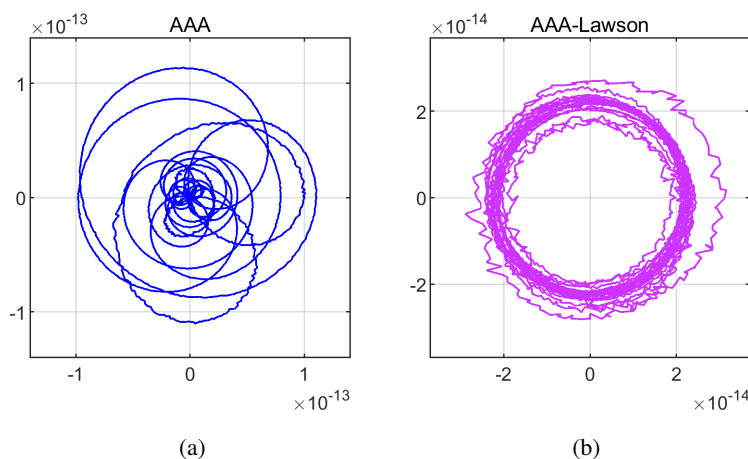
Figure 3.3. Error curves for AAA approximation of \Gamma(z) on the circle |z| = 1.5 : (a) straight AAA approximation, (b) AAA-Lawson approximation with 20 Lawson steps. The error curve has winding number 21 but is ragged because the errors are close to the level of machine precision (compare Figure 29.2). In this paper we use magenta to distinguish error curves from AAA-Lawson best approximation.
