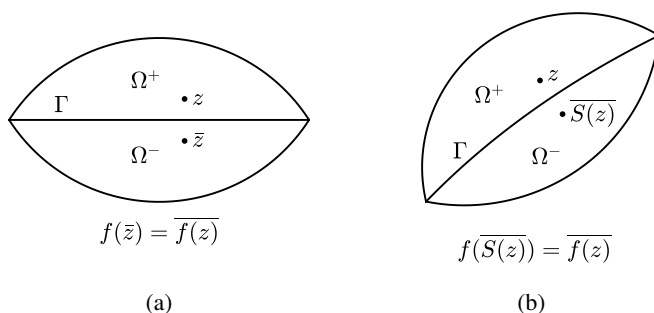
Figure 11.1. (a) The Schwarz reflection principle (Theorem 11.1) extends an analytic function that takes real values on a real interval across the interval from one half-plane to the other. (b) The generalization by the Schwarz function S(z) for reflection of an analytic function across an analytic arc \Gamma , again assuming it takes real values on \Gamma . This figure is not part of the governing Open Access licence for the article but has been reproduced from Trefethen (2025a), licensed under CC BY-SA 4.0, with permission from Springer Nature.
