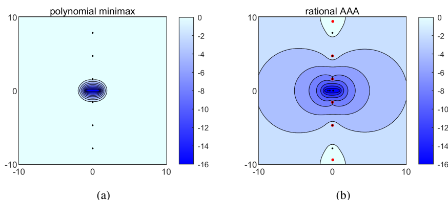
Figure 10.1. Numerical analytic continuation of \tanh(z) from data on [-1, 1] by (a) degree 30 polynomial minimax fitting and (b) degree 7 AAA rational fitting (error contours of \log_{10} |f(z) - r(z)| ). Black dots mark poles of f , and red dots mark poles of the rational approximation r . As is well known, polynomials have no accuracy beyond the first singularity, with ‘beyond’ and ‘first’ for this case of approximation on the interval defined by Bernstein ellipses surrounding [-1, 1] . Figure reproduced from Trefethen (2023), licensed under CC BY 4.0.
