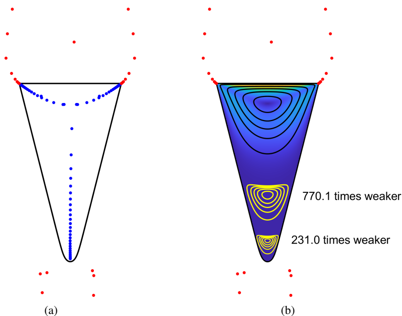
Figure 27.2. Stokes flow in another triangular driven cavity with a curved bottom computed by the AAALS Stokes method, following Xue, Waters and Trefethen (2024). As in Section 24, image (a) shows all the AAA poles and image (b) shows the poles outside the problem domain together with the computed solution. The poles placed by AAA are again clustered near the corners, but no longer lie on straight lines. The poles near the bottom are few, but still important for representing the solution to high accuracy. There are now two Moffatt eddies instead of an infinite sequence.
