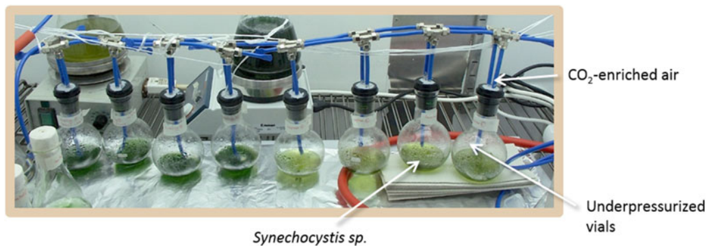
Fig. 5. Underpressurized culture vials used in Kirsi Lehto's laboratory (at the University of Turku, Finland) to grow cyanobacteria in low-pressure/high pCO 2 atmospheres.
