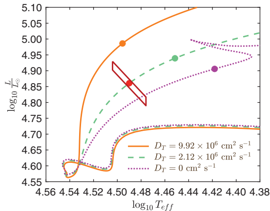
Figure 4. HR diagram for HD 152219: evolutionary tracks of Clés models. The dots over-plotted on the tracks correspond to the models that fit the observational \dot{k}_2 . The observational value and its error bars are represented in red.
