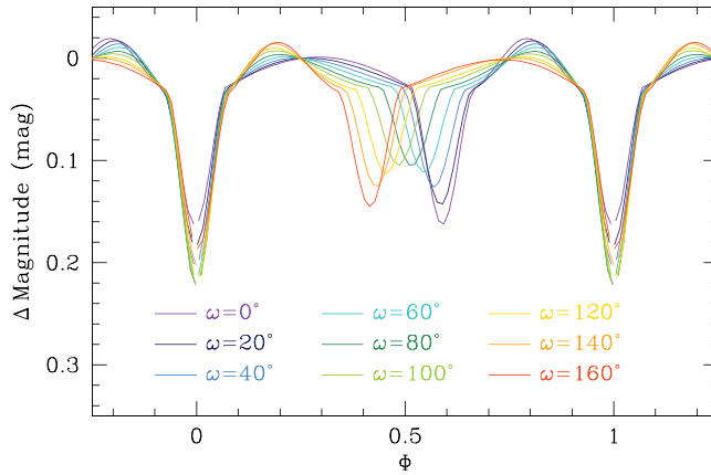
Figure 2. Set of theoretical light curves for different values of \omega , all other parameters being identical ( e = 0.134 , i = 68.6^\circ , and stars having the same m , R , and T_{\text{eff}} ). Figure from Rosu (2021).
