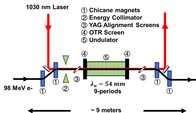
Figure 2. The configuration of the LCLS-II laser-heater system, which includes a 1030 nm laser, chicane magnets, optical transition radiation (OTR) screen, energy collimator, pop-in YAG alignment screens (to align the laser and the electron beam) and undulators [48,49] .
