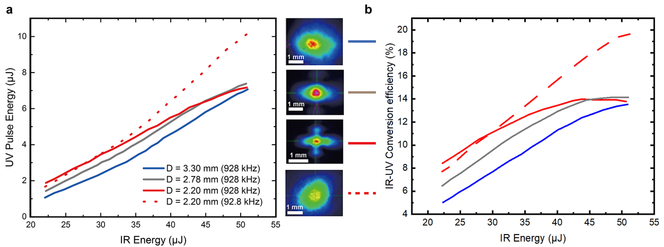
Figure 5. (a) UV pulse energy and (b) IR-UV conversion efficiency by optimizing the SHG beam size in the second SHG crystal. High repetition rates require finding a compromise among thermal stability, adequate spatial shape and conversion efficiency. Inset images show the transverse beam shapes from diameters 3.30 to 2.20 mm. IR-UV conversion efficiency across different SHG beam diameters in the second SHG crystal is at 928 kHz, with comparative data at 92.8 kHz for UV pulse energy and efficiency.
