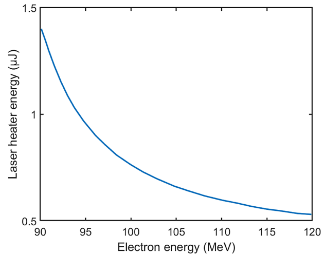
Figure 3. The calculated relationship between laser pulse energy and electron beam energy, specifically showcasing a 6 keV rms energy spread induced by the LH system in the case of a 100 pC bunch.
