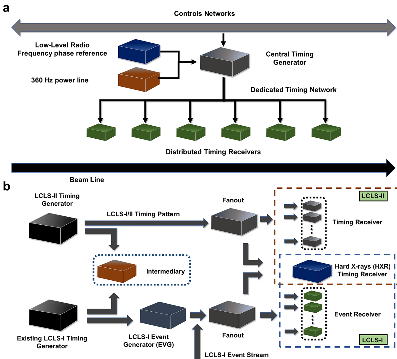
Figure 4. (a) Generic layout for a central timing generator distributing timing information to receivers distributed along the beam line. (b) Interoperability of the LCLS and LCLS-II timing systems (shown in Figure 1).
