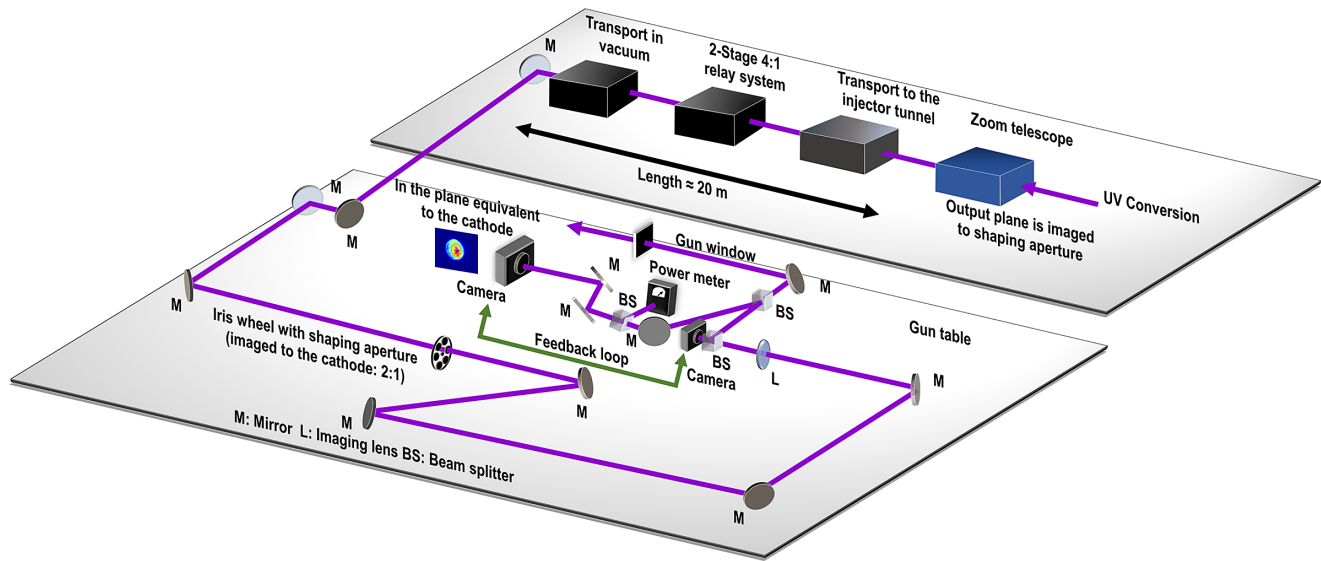
Figure 6. The laser beam transport system for the LCLS-II. Inset: the laser beam profile is monitored by the virtual cathode camera.
