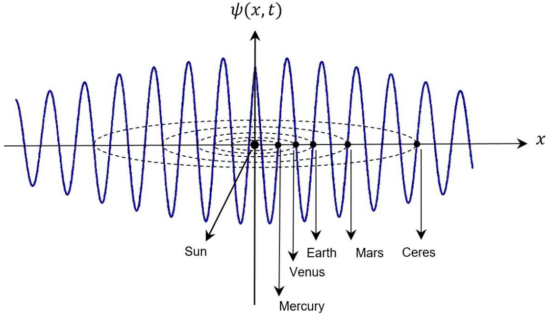
Fig. 1. Solar system standing wave packet with \lambda = 0.6 AU and \phi = \frac{\pi}{6} Diagram of \psi(x, t) at the moment t = 0 . The value of \psi(0,0) is equal to \sqrt{3}C/2 . This diagram is drawn by a certain value of C , \delta and \gamma in equation 1, which we will obtain their value at the end of the article. As you can see, the planets are on the nodes of the wave function. Jupiter, Saturn, Uranus, Neptune, and Pluto are on the nodes farther from the Sun.
