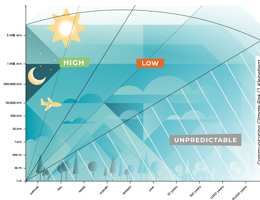
Figure 10. Illustrating how model prediction skill depends on spatial and temporal scales.
