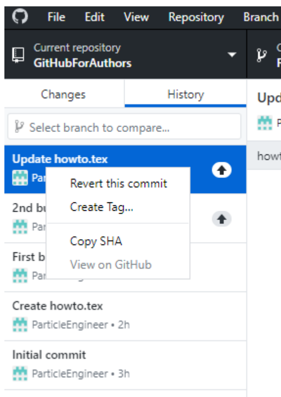
Figure 10: Reverting to a previous commit.
