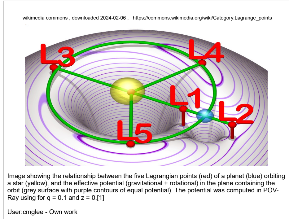
Figure 5: Lagrange points showcase from [43], wikimedia commons, thanks to user cmglee
