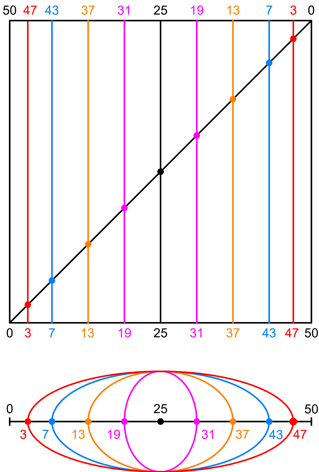
Figure 1. Partitioning the number 50 into pairs of prime numbers
