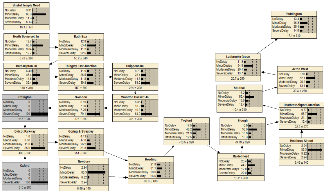
Figure 20: Bayesian network, with probability distributions learned from data augmented with heuristic and subjective probabilities where data sparse or non-existent. This shows the downstream effects on Paddington of a severe delay at both Uffington and Oxford, both feeding into Didcot Parkway. Image produced in Netica [5]
