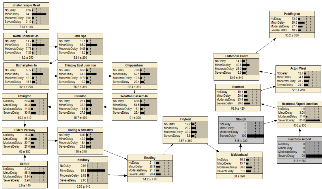
Figure 22: Bayesian network, with probability distributions learned from data augmented with heuristic and subjective probabilities where data sparse or non-existent. This shows the downstream effects on Paddington of a severe delay at both Slough and Heathrow Airport, both feeding into Heathrow Airport Junction. Image produced in Netica [5]
