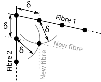
Figure 3: A schematic of the numerical construction of a grid of fibres.
