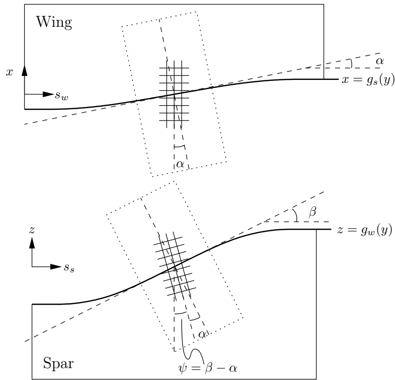
Figure 9: The rotation of the cells caused by a local straight fold at the wing-spar edge. Then the angle of the edge on the wing is \alpha and the angle of the edge on the spar is \beta , then the rotation of the mesh due to the fold over the edge is \beta - \alpha .
