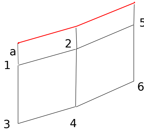
Figure 7: Flat spar solution: front view of the spar. The red line marks the edge between the spar and the wing cover.
