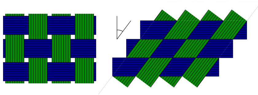
Figure 2: The simplest under-and-over carbon-fibre weave formed by ribbons comprising many individual fibres, initially crossing at right angles (left). Other weave patterns and initial fibre angles are also available. When subjected to simple shear, the gaps between the ribbons are reduced. The critical shear occurs when the ribbons come into contact (right).
