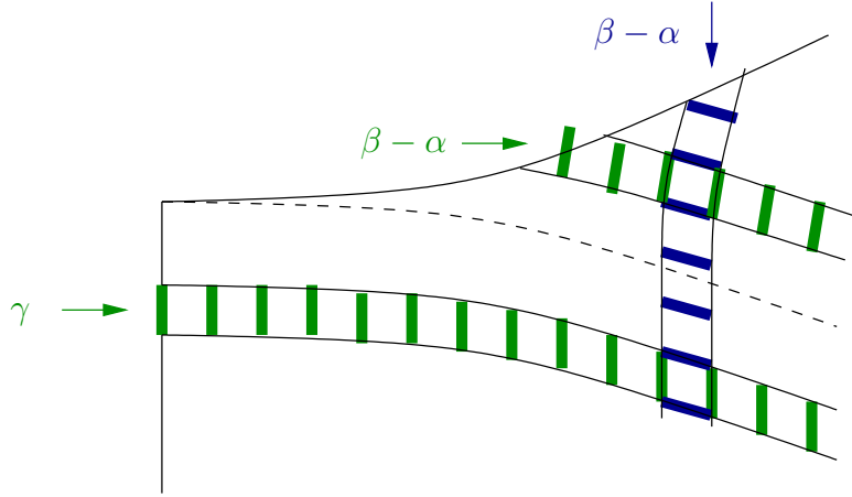
Figure 8: In each row or column of cells on the spar, the transverse ribbons segments must remain parallel. Therefore the rotation of the horizontal ribbon segments (blue) in each column of cells is set by the conditions at the wing edge, while the rotation of the vertical ribbon segments (green) in each row is set either by the left-hand boundary or by the conditions at the wing edge, depending on where the horizontal ribbon originated.
