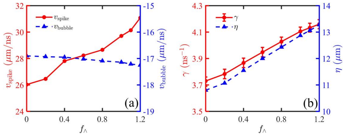
FIG. 7. At t = 2.0 \text{ ns} , (a) the velocity of the spike tip (red-circle line) and the bubble vertex (blue-delta line), and (b) the linear growth rate (red-circle line) and the amplitude (blue-delta line) for different f_{\Lambda} factor.
