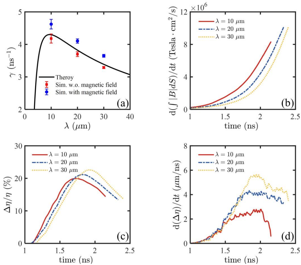
FIG. 9. (a) The comparison of the linear growth rate. The black-solid line is the theoretical prediction. The red-circles are from the simulations without magnetic field and the blue-squares correspond to the cases with magnetic field included. The generation rate of the self-generated magnetic field(b), the percentage increase (c) and the derivative of the amplitude difference (d) evolve over time for different wavelengths.
