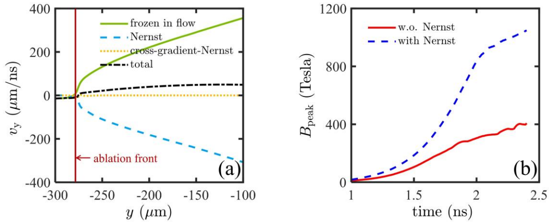
FIG. 8. (a) The distributions of y-component of the fluid velocity (green-solid line), the Nernst advection velocity (blue-dashed line) and the cross-gradient-Nernst velocity (yellow-dot line) and the total velocity (black-dashed-dot line), which are diagnose at the right side of the spike x = 5.0 \mu\text{m} at t = 2.0 \text{ ns} . (b) The peak magnitudes of magnetic field evolve over time without (red-solid line) and with the Nernst effect (blue-dashed line).
