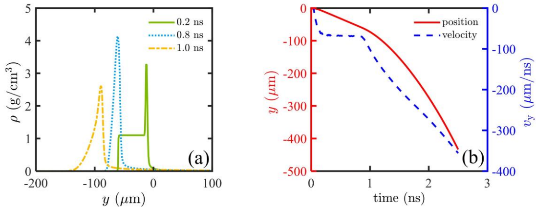
FIG. 2. (a) The density distribution along y -axis at different times. (b) The position (red-solid line) and velocity (blue-dashed line) of the ablation front evolve over time.
