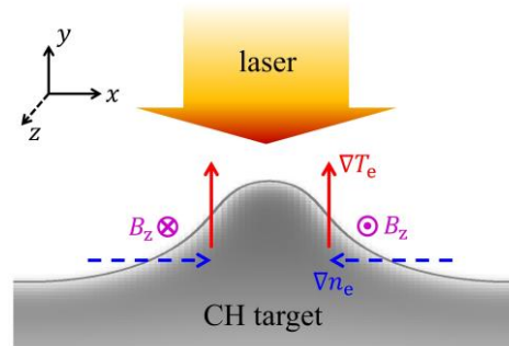
FIG. 1. Schematic diagram of a laser driven the RTI with the self-generated magnetic field included.
