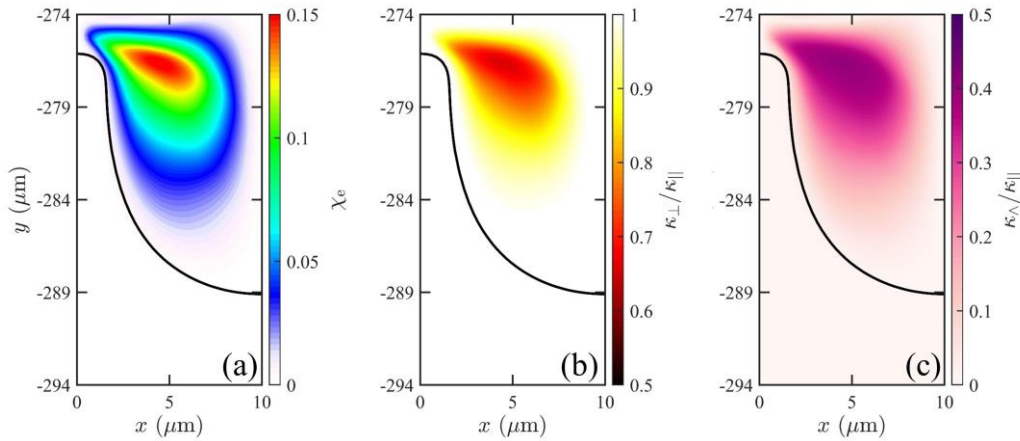
FIG. 5. The spatial distributions of (a) Hall parameter \chi_e , (b) the ratio of perpendicular to parallel thermal transport coefficients \kappa_{\perp}/\kappa_{\parallel} and (c) the ratio of cross to parallel thermal transport coefficients \kappa_{\Lambda}/\kappa_{\parallel} at t = 2.0 ns. Only the right side of the spike is shown.
