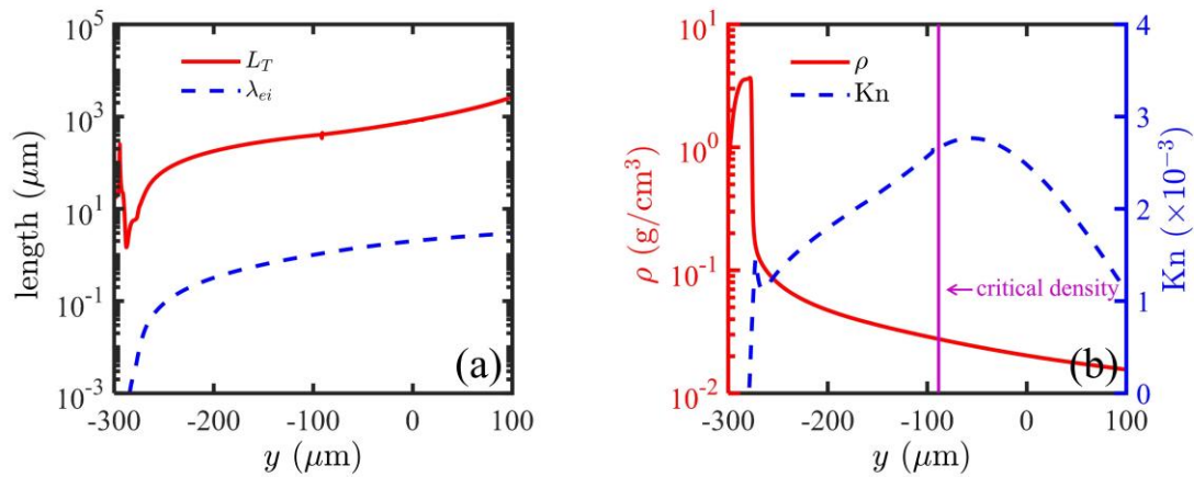
FIG. 10. At t = 2.0 ns, (a) the distributions of the temperature gradient scale length L_T (red-solid line) and the electron mean free path \lambda_{ei} (blue-dashed line), (b) the density (red-solid line) and the Knudsen number (blue-dashed line) along y-axis, which are diagnosed at x = 0 . The pink-solid line in Figure 10(b) represents the critical density surface.
