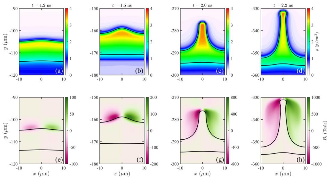
FIG. 3. The spatial distributions of the density (a-d) and the magnetic field (e-h) at different times during the evolution of RTI.
