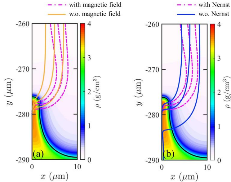
FIG. 6. At t = 2.0 ns, a comparison of heat flux streamlines with (without) magnetic field (a), and with (without) Nernst effect (b) is overlaid on the density spatial distribution. Only the right side of the spike is shown. The pink-dashed-dot lines in Figure 6(a) and Figure 6(b) are identical.
