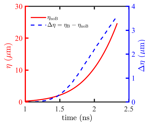
FIG. 4. The peak-to-valley amplitude evolves over time without magnetic field (red-solid line). The blue-dashed line is the amplitude difference between the amplitude with and without the magnetic
