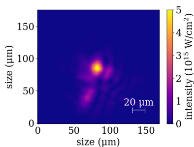
Figure 11. Intensity distribution in the focal spot of the PHELIX beam at HHT.
