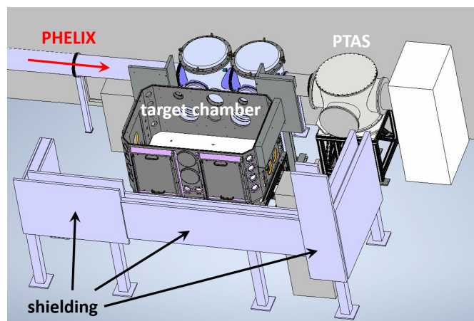
Figure 8. 3D-model of the Petawatt Target Area served by PHELIX. The target chamber has two entrance possibilities for the laser beam(s), which allows to accommodate very diverse and highly complex experimental setups.
