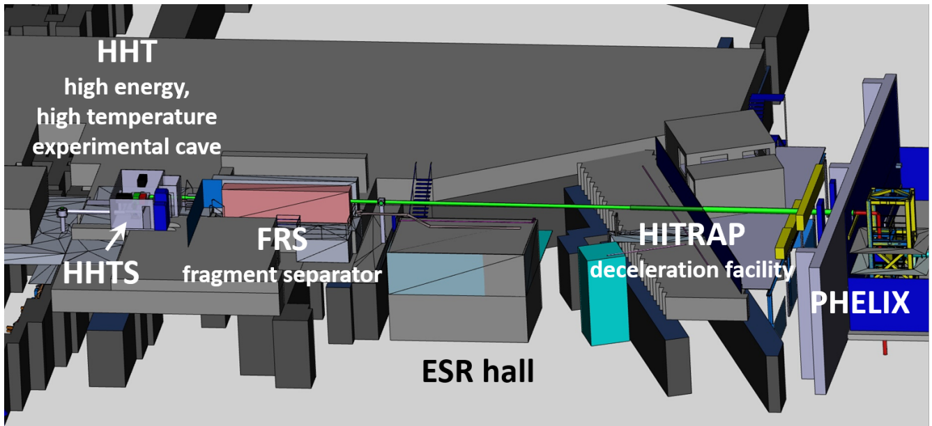
Figure 2. Digital mock-up of the experimental hall (ESR hall) downstream of the SIS18 heavy-ion synchrotron, showing the PHELIX beamline (green/grey tube) as it traverses several experimental areas on its way to HHT. The total length of the beam transport is on the order of 65 m.
