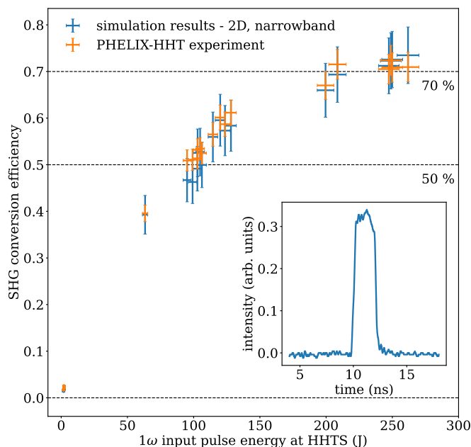
Figure 10. Second-harmonic generation in the PHELIX-HHT beamline showing the conversion efficiency at HHTS. The inset shows a temporal shape of the PHELIX narrowband pulse.
