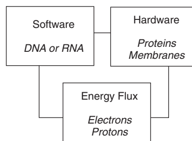
Fig. 1. A tripartite description of life on Earth, based on Schrödinger (1944) and von Neumann (1951, 1966). All three components are necessary, but not sufficient: thermodynamic considerations dictate that for a living entity to perpetuate it must also replicate.
