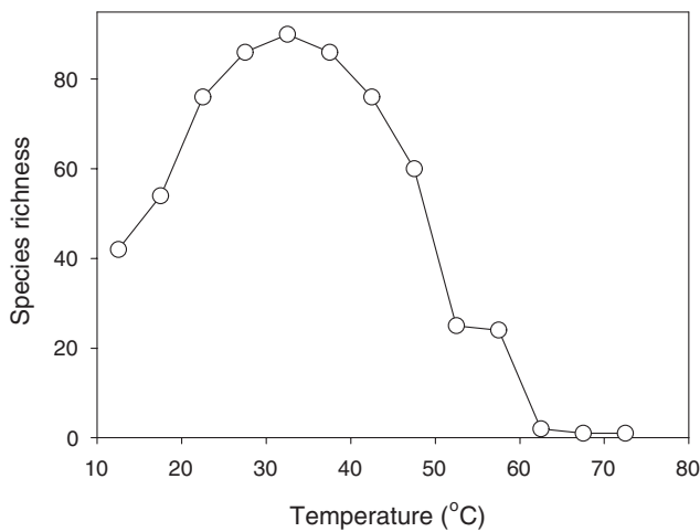
Fig. 3. Species richness (number of species) of cyanobacteria as a function of water temperature across a range of geothermally heated pools in Yellowstone National Park. Replotted from data in Brock (1978).
