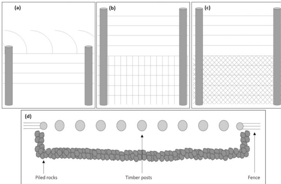
FIG. 1 The three fence structures used on two wildlife properties in Laikipia County, northern Kenya, referred to here as Property A and Property B: (a) Type A1 fence, which surrounds Property A1; (b) Type A2 fence, which surrounds Property A2; (c) Type B fence, which surrounds Property B; and (d) design of the fence gaps.
