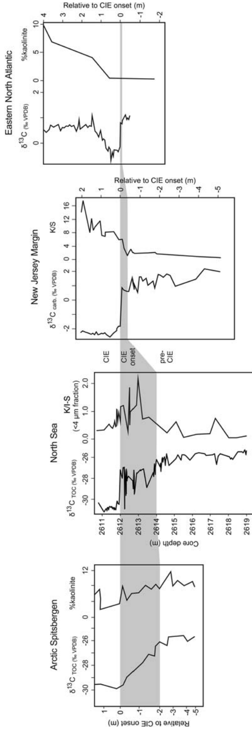
FIG. 9. Comparison of kaolinite (this study) and sediment carbon isotope (from Kender et al. , 2012) from 22/10a-4 with recent studies from Arctic Spitsbergen (Harding et al. , 2011), New Jersey Margin (John et al. , 2012) and the Eastern North Atlantic (Bormemann et al. , 2014).
