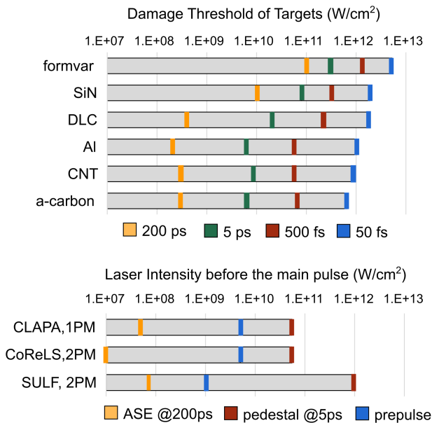
Figure 5. Comparison between DTIs of the tested ultrathin foils and the prepulse intensity.
