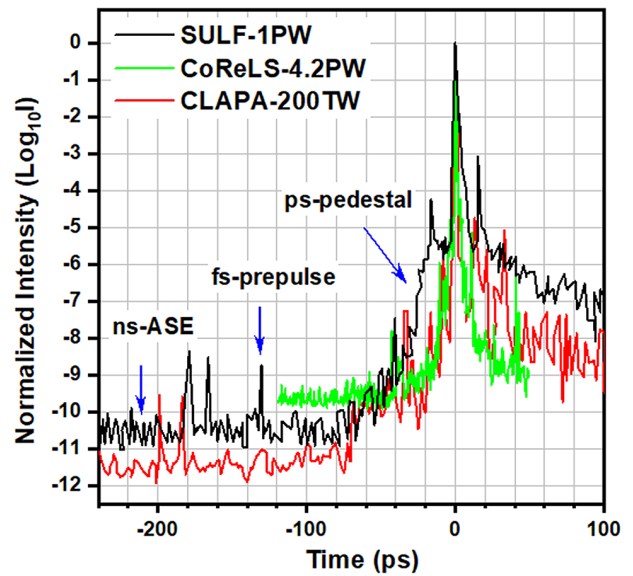
Figure 4. The temporal profiles of three ultraintense femtosecond laser pulses from the SULF, CoReLS, and CLAPA facilities, respectively.
