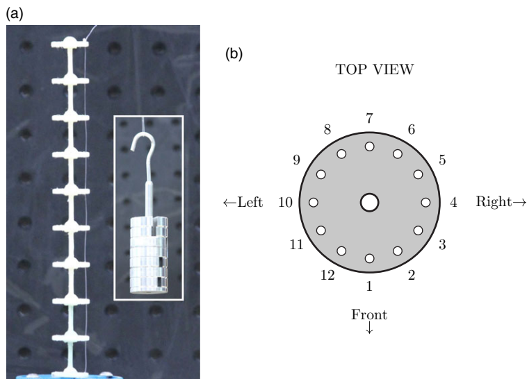
Figure 4. (a) Experimental setup for straight routing with the load shown in the inset. (b) Top view of the holes on a disk showing the numbering scheme.
