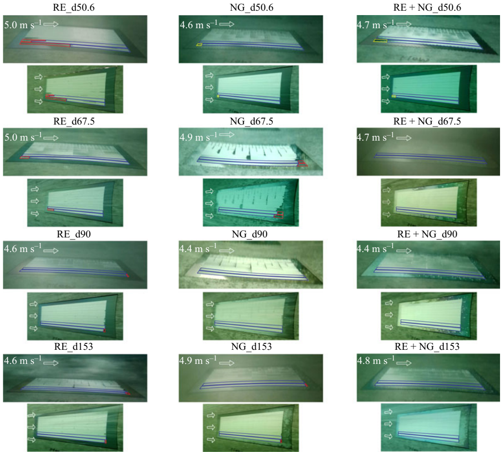
Figure 11. Sample images at speeds in the range 4.4–5 \text{m s}^{-1} . Blue indicates a pinned or slightly depinned interface (i.e. h/w \leq 0.17 ); yellow indicates a depinned interface (i.e. 0.17 < h/w < d/w ); and red indicates no interface (i.e. h/w = d/w ).
