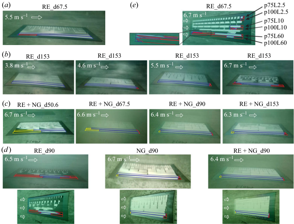
Figure 6. Sample images for key trends. Some regions are colour-outlined to help identify the plastron states, which were determined using the corresponding image pairs in Appendix E. Blue, yellow and red indicate the pinned or slightly depinned interface (i.e. h/w \leq 0.17 ), depinned interface (i.e. 0.17 < h/w < d/w ) and no interface (i.e. h/w = d/w ), respectively. (a) The effect of trench width w shown by the side camera. Narrower trenches maintained the plastron better. (b) The effect of shear stress \tau_w shown by the side camera. Slower flows maintained the plastron better. (c) The effect of trench depth d shown by the side camera. Deeper trenches maintained the plastron better. (d) The effect of nano-grass shown by the two cameras. For each pair of images, the top image was taken by the side camera, and the bottom image was taken by the rear camera. While the plastron was lost significantly on RE at this high flow speed ( U = 6.4\text{--}6.7\text{ m s}^{-1} ), a pinned or slightly degraded plastron was found for all trenches on NG and RE + NG, demonstrating the effectiveness of adding nano-grass. (e) Effects of dynamic water pressure and interfacial contamination shown by the rear camera. Regions with trench length L = 2.5\text{ mm} , 10\text{ mm} , and 60\text{ mm} are outlined. The inset picture shows the pinned or slightly depinned interfaces at the front end of the 60\text{ mm} trenches.
