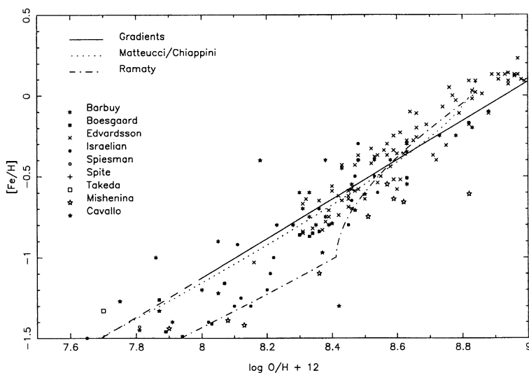
Figure 2. The [\text{Fe}/\text{H}] \times \log(\text{O}/\text{H}) relation in the galactic disk.
