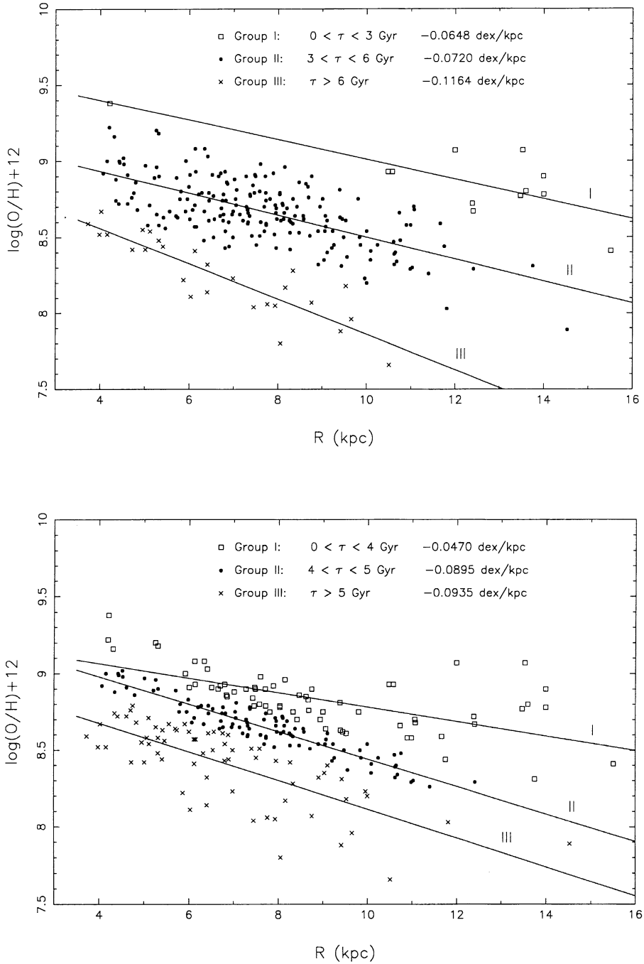
Figure 1. Time variation of the O/H gradient from PN.
