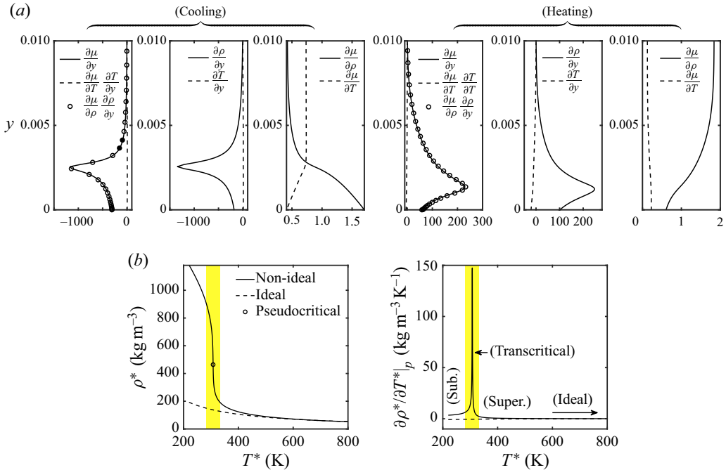
Figure 16. (a) The y-gradient of viscosity in the transcritical regimes with wall cooling and heating; (b) density \rho^* and its gradient \partial\rho^*/\partial T^*|_p versus temperature at p^* = 80 bar. The yellow shaded area stands for strong gradients of thermodynamic properties near the Widom line (pseudocritical point).
