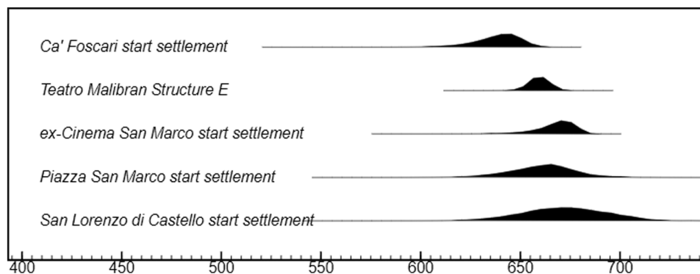
Figure 4. Estimated start of settlement at five locations in central Venice, based on the Bayesian chronological models in Meadows et al. (2012) and the online supplementary information (the Teatro Malibrán date is for the cross-matched timber structure shown in Figure 3) (figure by J. Meadows).
