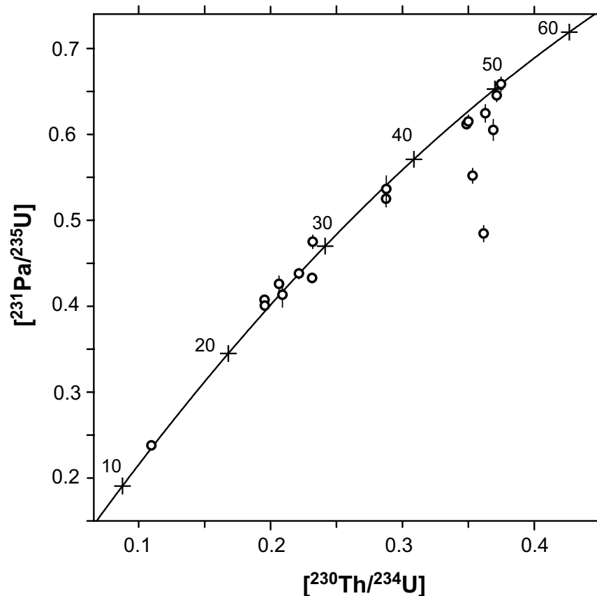
Figure 5 ^{231}\text{Pa} - ^{230}\text{Th} concordia diagram. [^{231}\text{Pa}/^{235}\text{U}] - [^{230}\text{Th}/^{234}\text{U}] concordia diagram of samples analyzed for ^{231}\text{Pa} . All samples are from Papua New Guinea; error bars are 2\sigma and, if not visible, are smaller than the symbol. The curved line, "concordia," shows equal ^{231}\text{Pa} - ^{230}\text{Th} age values. Crosses on concordia indicate age in thousands of years (kyr).
