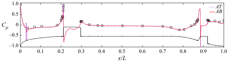
Figure 21. Profiles of C_p along the upper meridian (the hull profile displayed in the figure, corresponding to z = 0, y \geq 0 ) for cases AT and AB , along with LES results of Posa & Balaras (2016) (•, grey) and the experimental C_p of Liu & Huang (1998) (□) from pressure taps at locations shown as dots on the hull profile. Note that the C_p from Posa & Balaras (2016) is from the hull surface only (not from the sail or stern appendage), and therefore is not plotted over these appendages.
