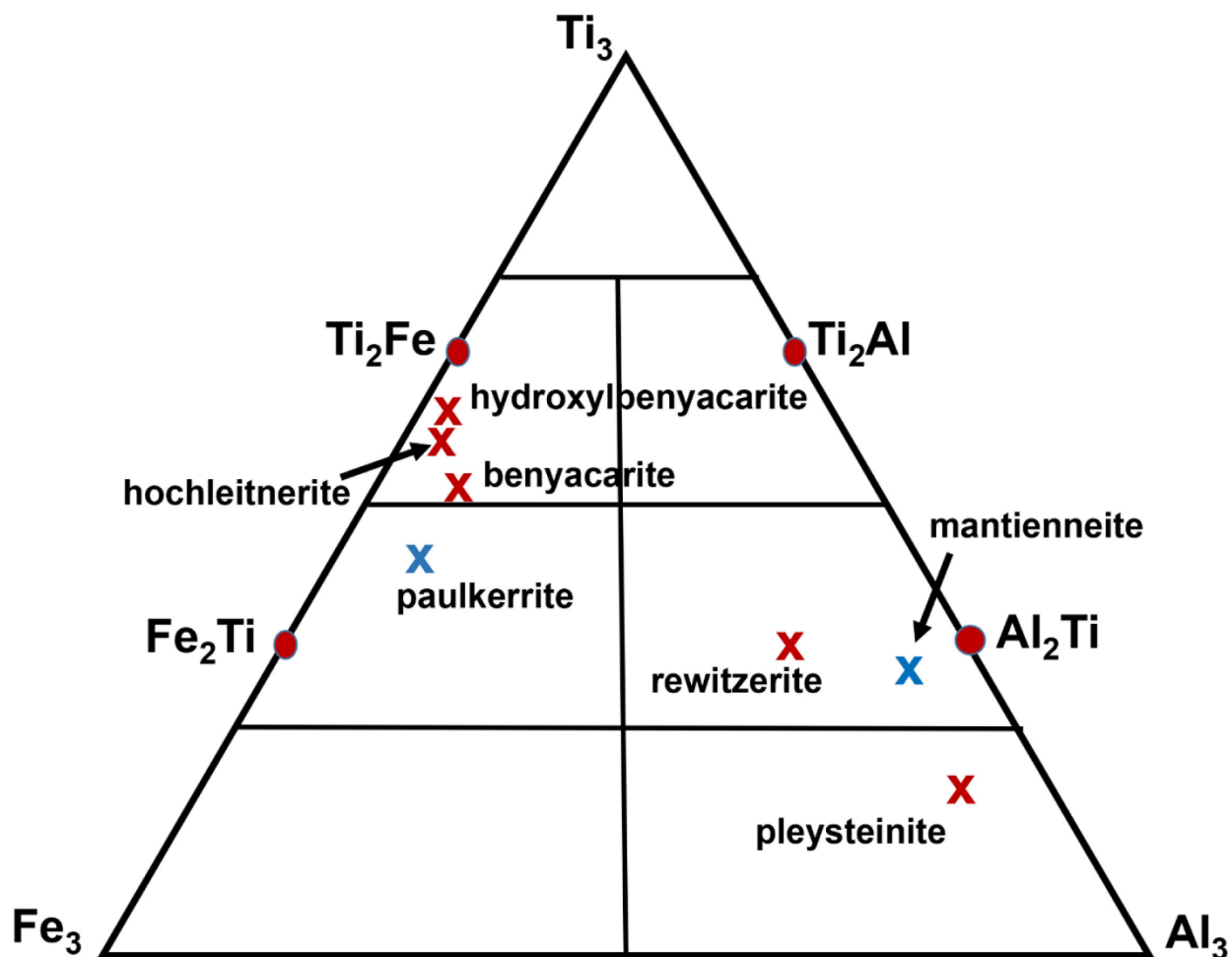
Figure 3. Ternary diagram for merged ( M_2M_3 ) site Al-Ti-Fe 3+ compositions, showing end-member compositions (Al 2 Ti, Ti 2 Fe etc) and location of the experimental compositions for benyacarite and hydroxylbenyacarite. Blue crosses have Mg at M_1 and red crosses have Mn at M_1 .
