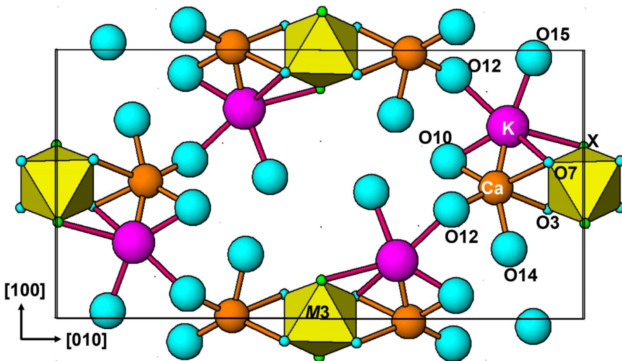
Figure 6. (001) section of the hydroxylbenyacarite structure at z = 0 , showing in-section bonds to Ca and K.
