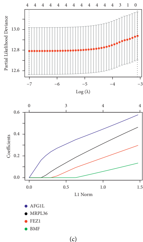
FIGURE 1: Screening of mitochondria-related genes and establishment of a risk score model. (a) Differential (increased or reduced) mitochondria-related gene expression in the hazard group compared with that in the normal group. (b) Error rates of randomly generated trees (upper panel). Variable relative importance of the four selected mitochondria-related genes. (c) LASSO analysis: partial likelihood deviance values were plotted against \log(\lambda) (upper panel). The relative abundance of the selected genes varies with the risk score.
