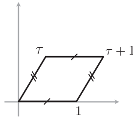
Figure 1.2 Fundamental region for the identification (5.3.64) defining a torus. The sides marked by the same symbol are to be considered as identified.
