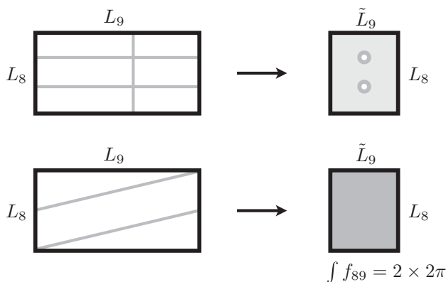
Figure 1.1 T-duality acting on D1-branes on a T^2 . It maps horizontal and vertical D1-branes to D0- and D2-branes respectively; it maps oblique D1s to D2/D0 bound states.
